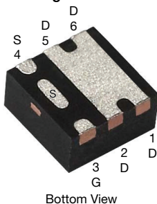
PowerPAK® SC-70-6L Single
