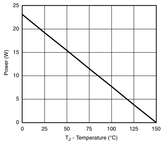
Power Derating
