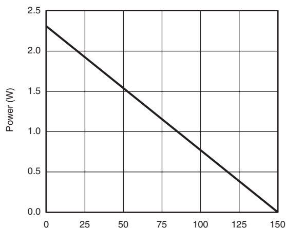
Power, Junction-to-Ambient
