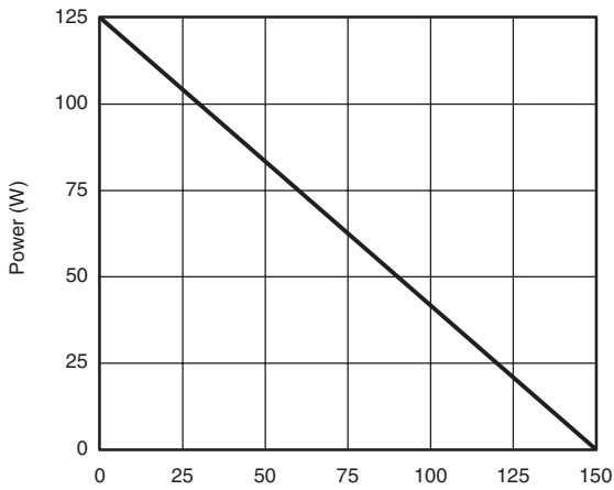
Power, Junction-to-Case
