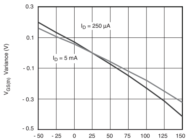
Threshold Voltage
