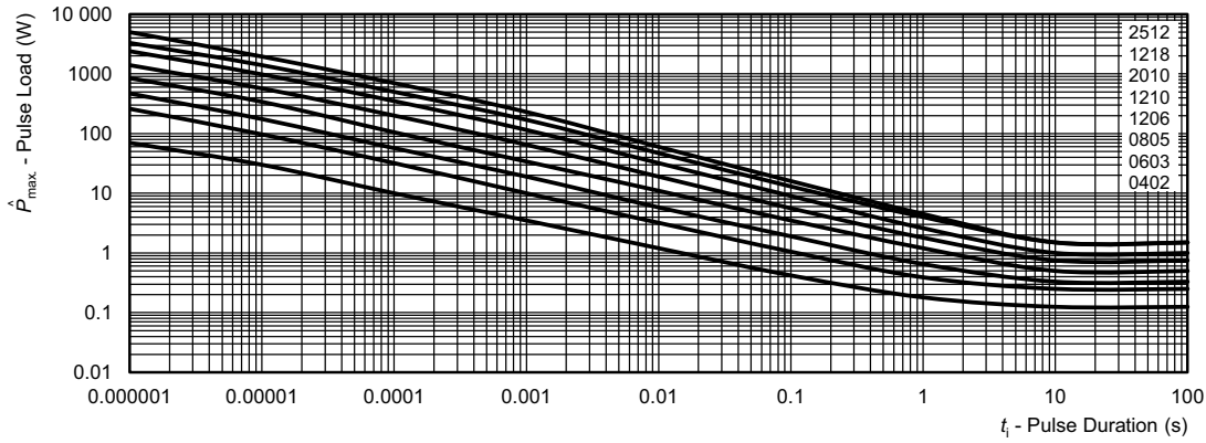
Maximum pulse load, single pulse; applicable if \bar{P} \rightarrow 0 and n < 1000 and \dot{U} \leq \dot{U}_{max} ; for permissible resistance change equivalent to 8000 h operation
