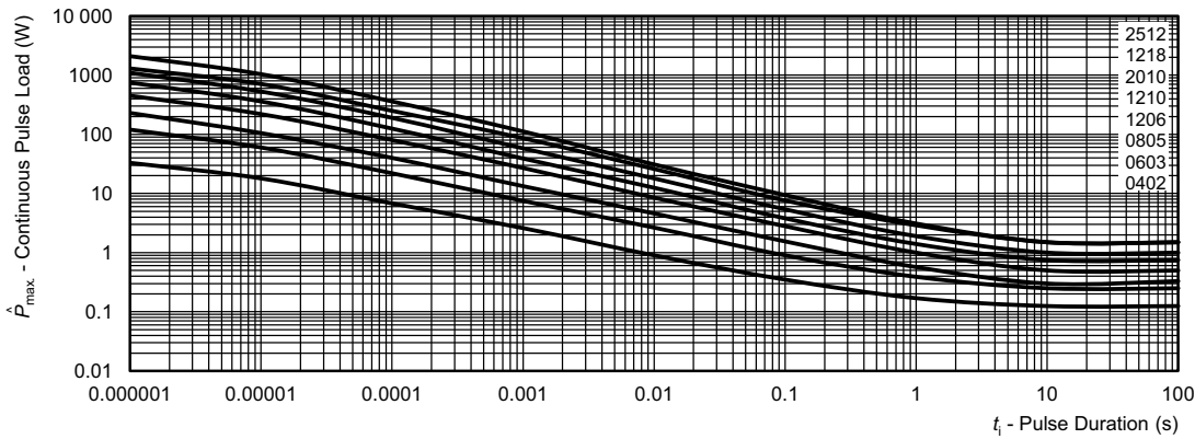
Maximum pulse load, continuous pulses; applicable if \bar{P} \leq P(\theta_{amb}) and \dot{U} \leq \dot{U}_{max} ; for permissible resistance change equivalent to 8000 h operation
