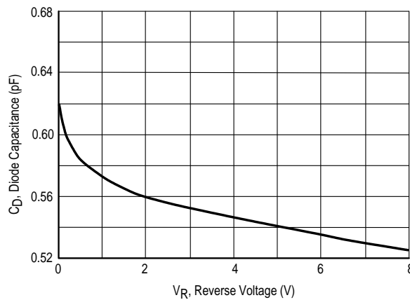
Figure 4. Capacitance
