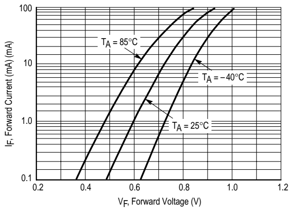
Figure 2. Forward Voltage
