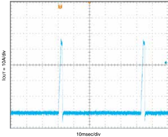
Short Circuit Current ( V_{IN} = 12V , V_{OUT} = 0.75V )
