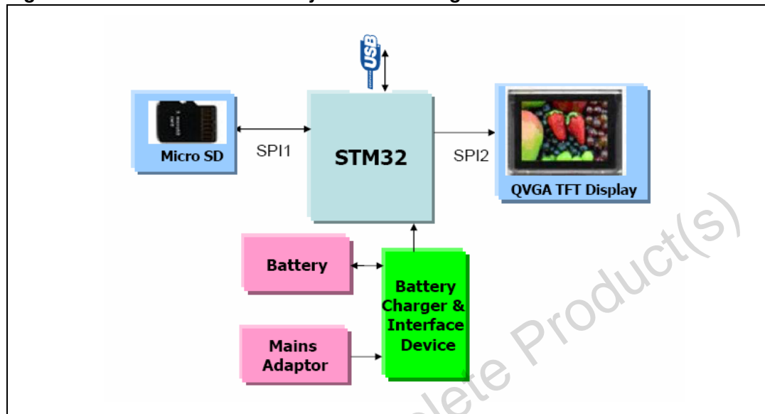
Figure 1. STEVAL-CCM001V1 system block diagram
