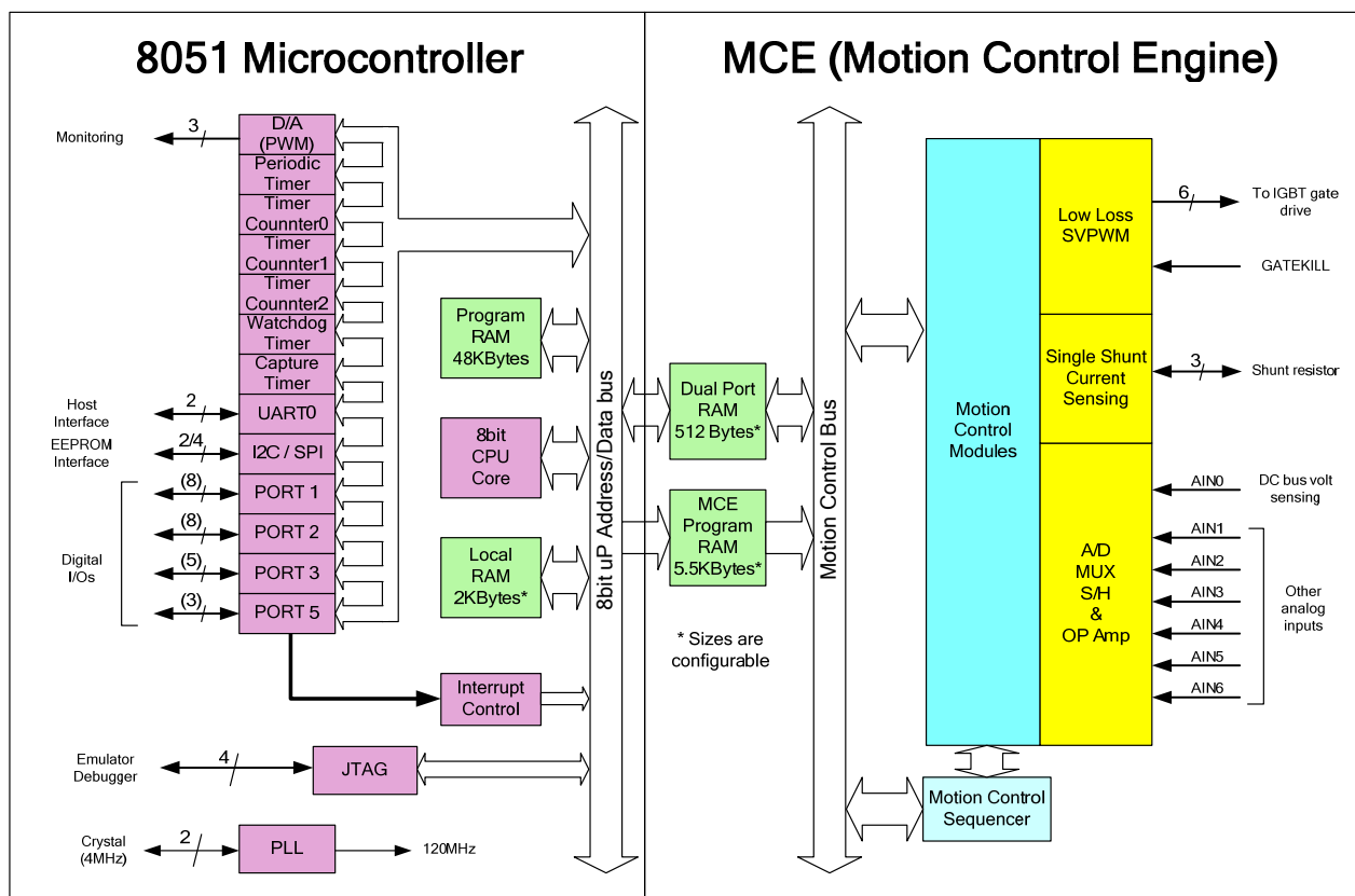
Figure 2. IRMCF341 Internal Block Diagram
