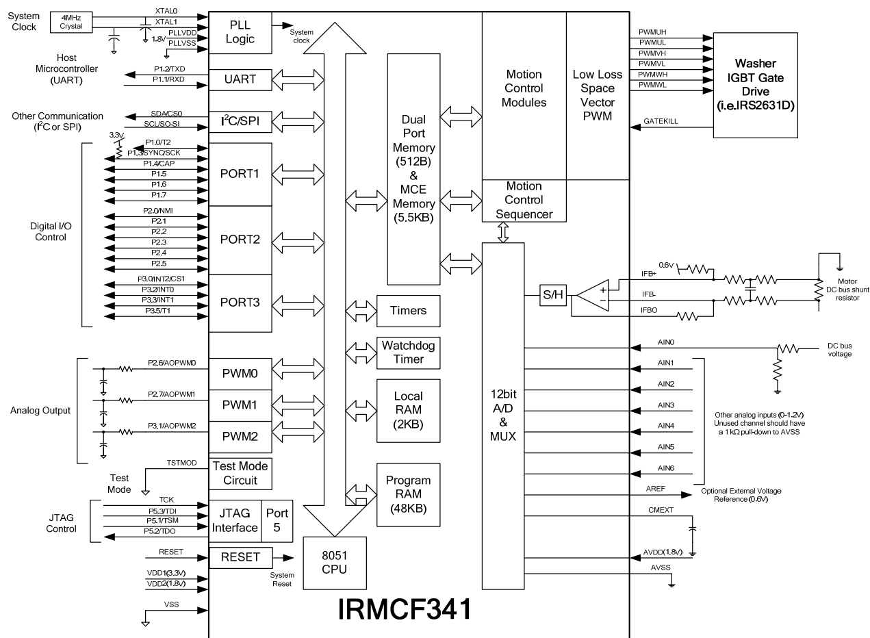
Figure 5. Application Connection of IRMCF341
