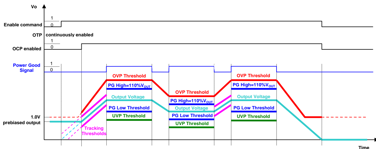
Figure 42. Protection Enable Conditions
