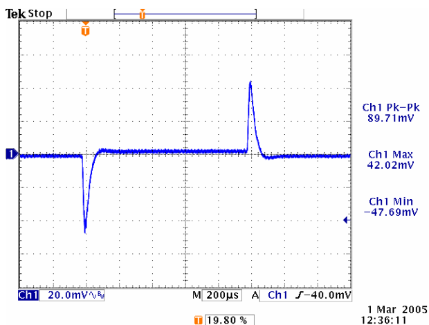
Figure 19. Vin=12V, Vout=1V, BW~60kHz.
