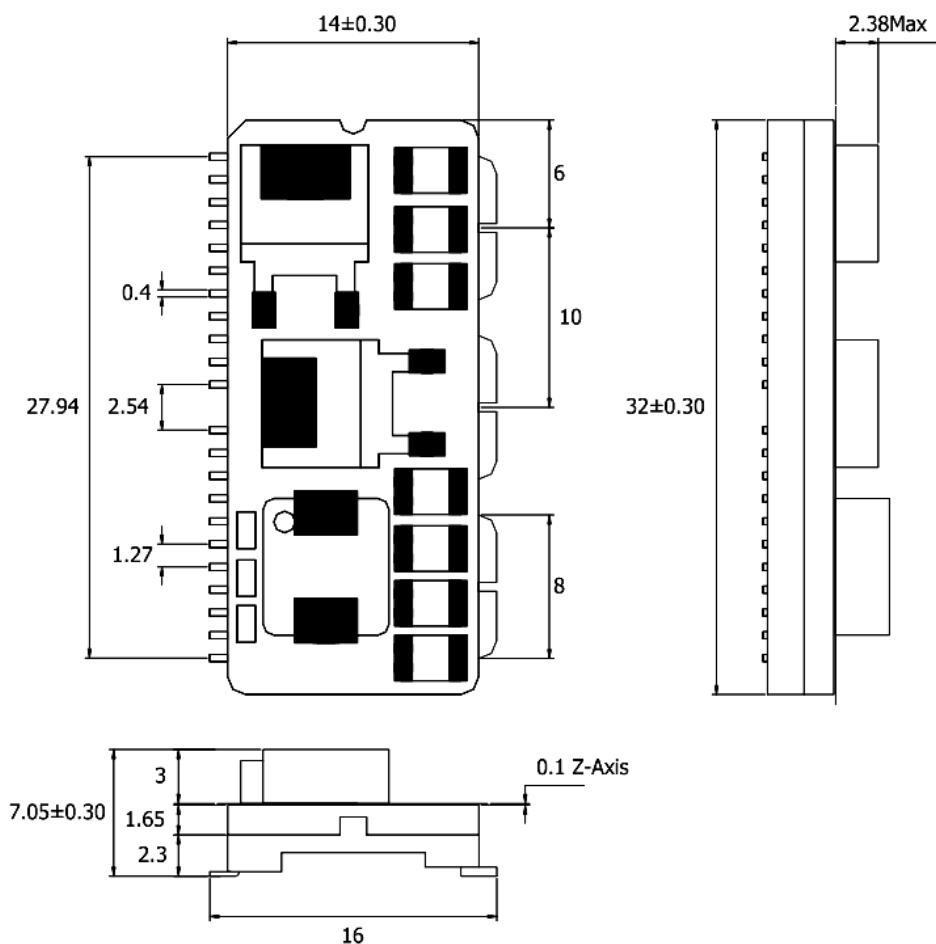
Figure 57. Mechanical Drawing
