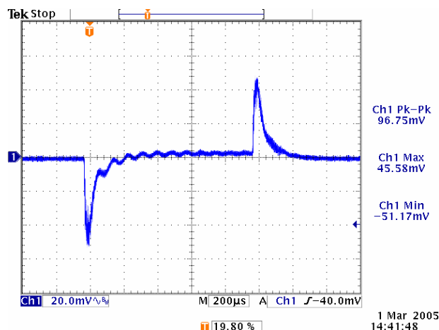
Figure 20. Vin=5V, Vout=2.5V, BW~60kHz.
