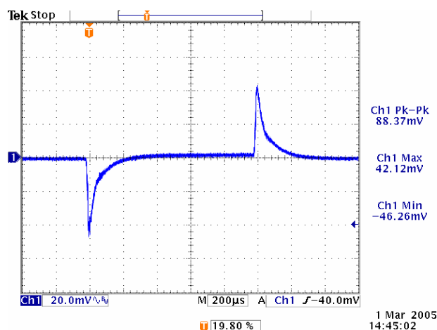
Figure 21. Vin=5V, Vout=1V, BW~60kHz.
