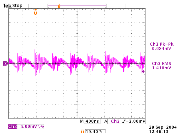
Figure 52. Output Voltage Noise, Full Load, 180° Interleave
