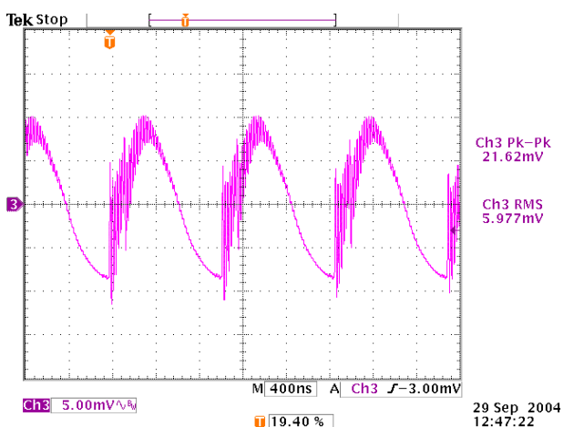
Figure 51. Output Voltage Noise, Full Load, No Interleave
