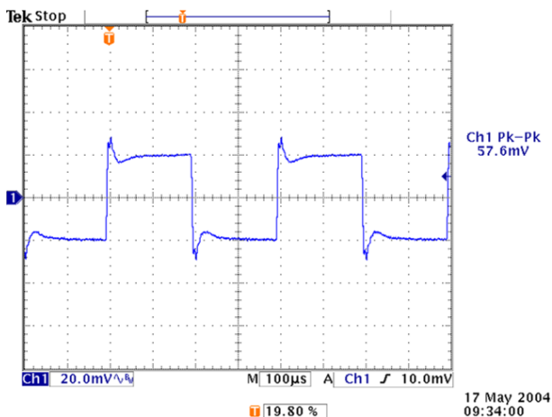
Figure 31. Transient Response with Optimal Voltage Positioning
