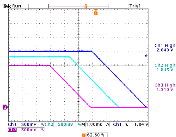
Figure 17. Turn-Off with Tracking and Sequencing. Falling Slew Rate with Tracking and Sequencing. Programmed at 0.5V/ms. Vin=12V, Ch1 - V1, Ch2 - V2, Ch3 - V3
