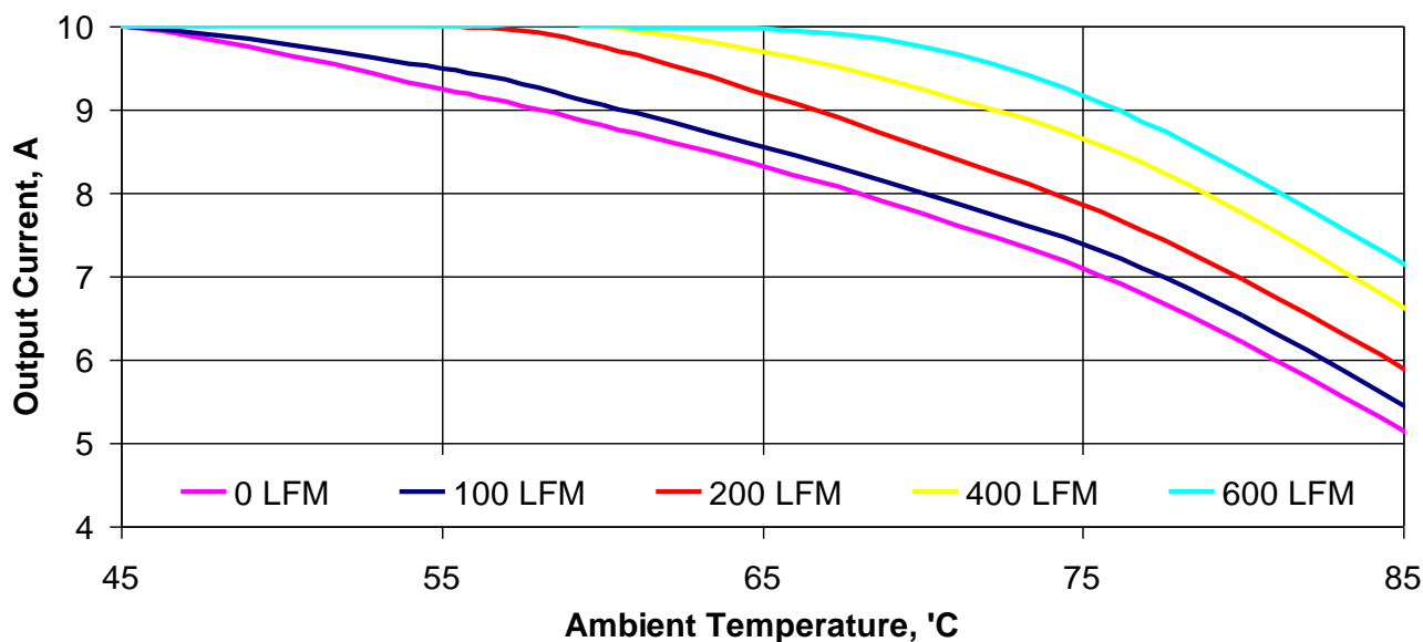
Figure 24. Thermal Derating Curves. Vin=13.2V, Vout=5.0V, Fsw=1MHz
