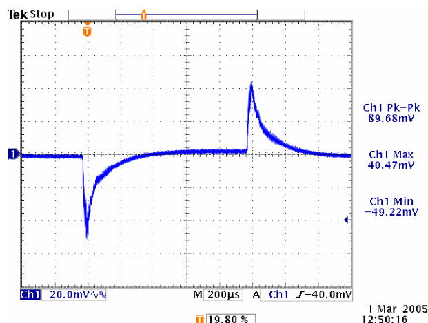
Figure 22. Vin=3.3V, Vout=1V, BW~60kHz.
