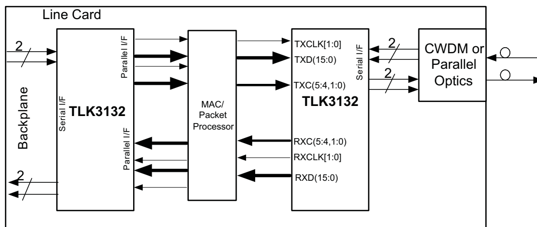
Figure 1-1. System Block Diagram – PCS
