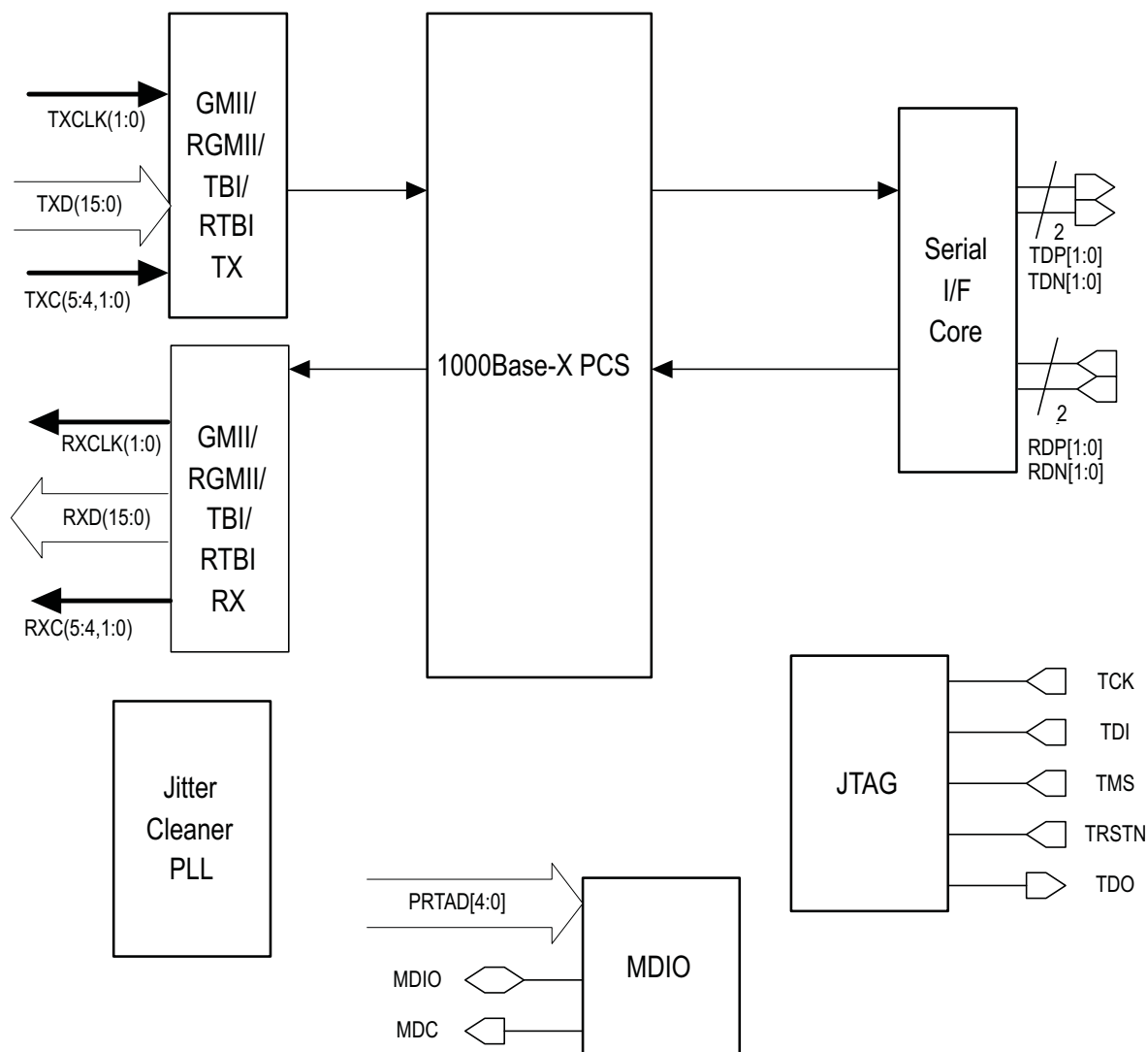
Figure 2-5. TLK3132 Block Diagram
