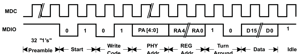
Figure 2-23. CL22 - Management Interface Write Timing
