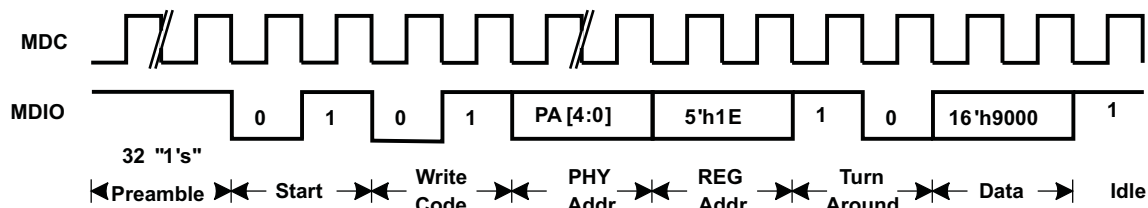
Figure 2-26. CL22 – Indirect Address Method – Address Write
