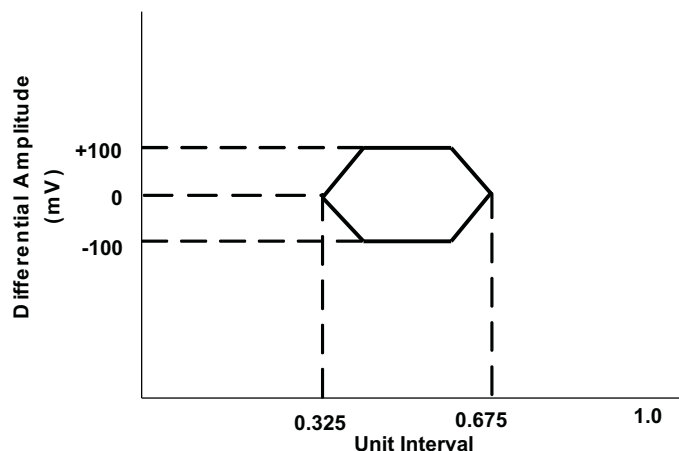
Figure 4-3. Receive Template
