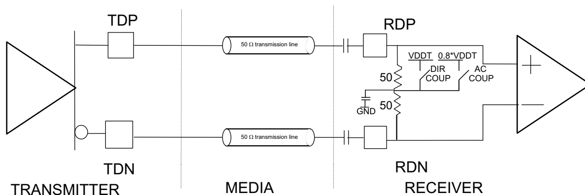
Figure 2-20. Example High-Speed I/O AC Coupled Mode
