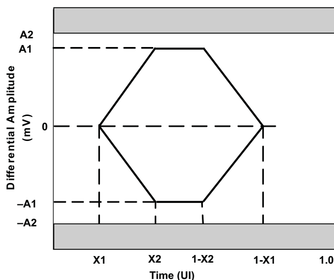
Figure 4-2. Transmit Template
