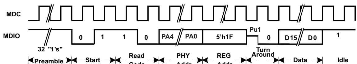
Figure 2-27. CL22 – Indirect Address Method – Data Read
