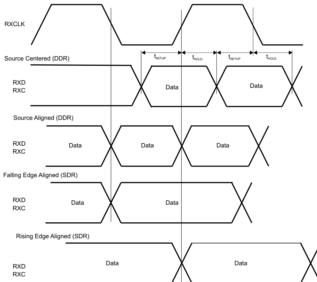
Figure 2-18. Receive Interface Timing – Source Centered/Aligned
