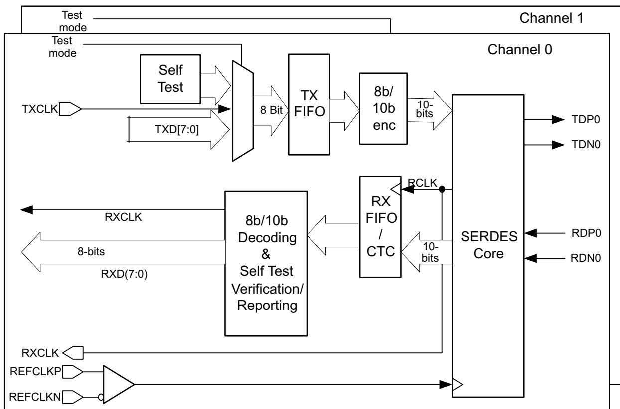
Figure 2-6. Detailed 1000Base-X Core Block Diagram
