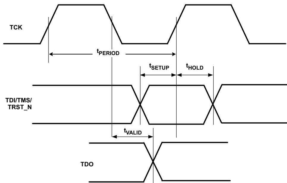
Figure 4-14. JTAG Timing
