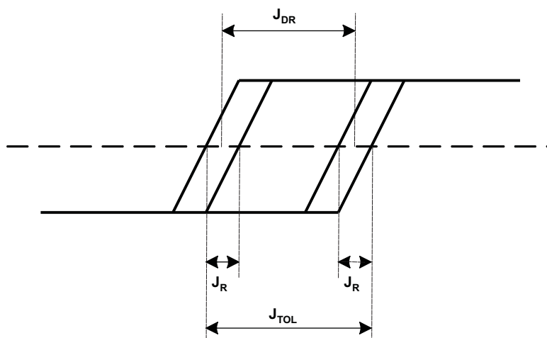
Figure 4-4. Input Jitter
