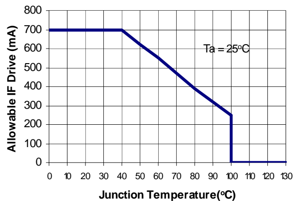
Derating Curve/die
