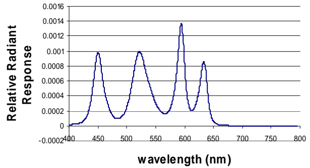
Spectral Responses for CRI 90 ( varied RGB I F Drives)
