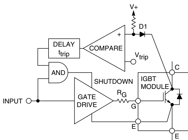
Figure 1. Desaturation Detector
