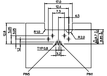
RECOMMENDED PCB LAYOUT - TYPE 'B' (TOP VIEW, COMPONENT SIDE)
