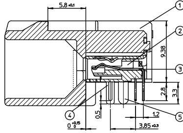
SECTION Z-Z
