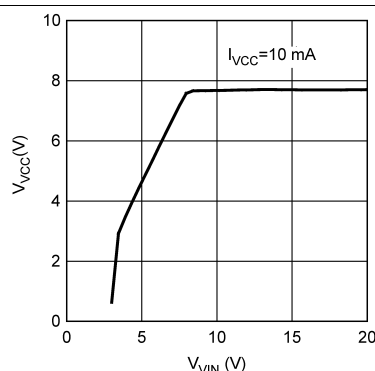
Figure 2. V_{CC} vs V_{IN}
