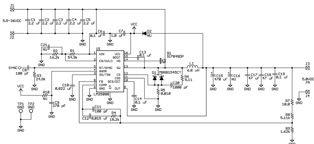
Figure 27. LM25088-1 Application Schematic
