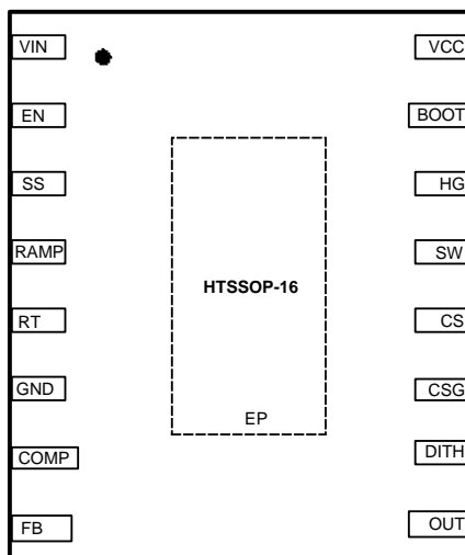
LM25088-1 16 Pin PWP Package (Dither Version) (Top View)
