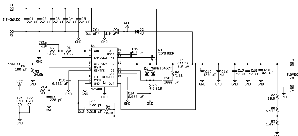
Figure 28. LM25088-2 Application Schematic
