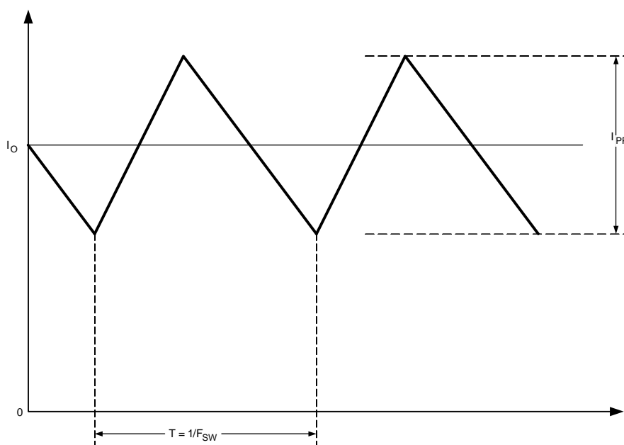
Figure 22. Inductor Current
