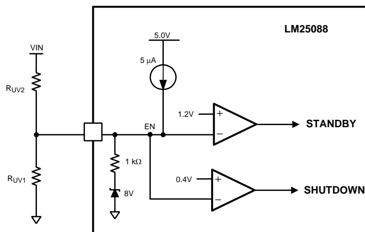
Figure 14. Basic Enable Configuration
