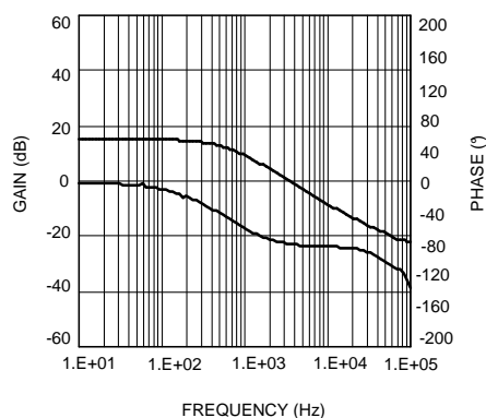
Figure 24. Modular Gain Phase
