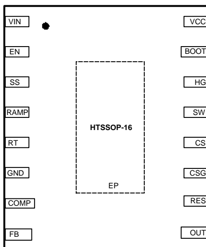
LM25088-2 16 Pin PWP Package (Restart Version) (Top View)
