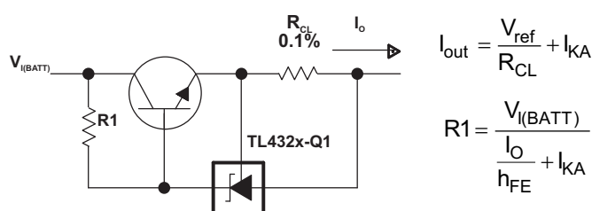
Figure 28. Precision Current Limiter
