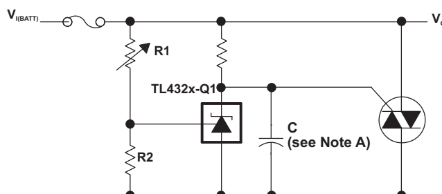
Figure 22. Crowbar Circuit
