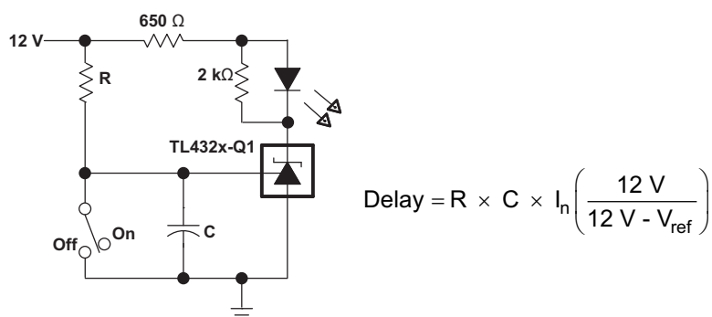
Figure 27. Delay Timer
