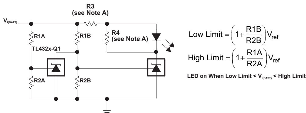
Figure 26. Voltage Monitor
