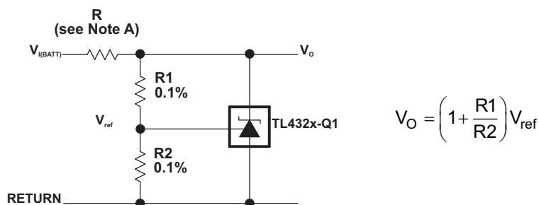
Figure 17. Shunt Regulator
