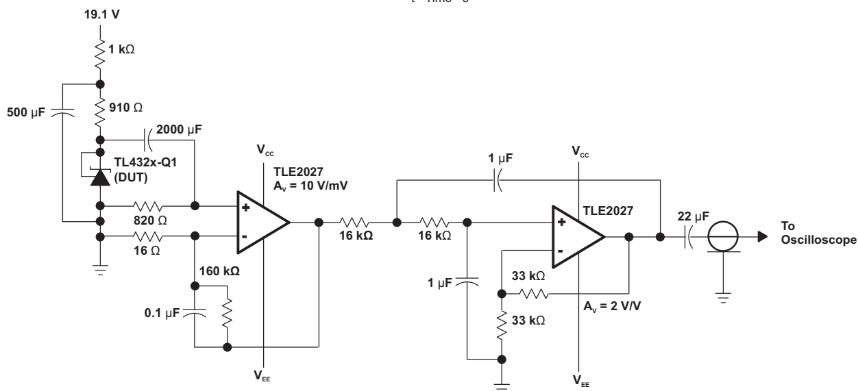
Figure 12. Test Circuit for Equivalent Input Noise Voltage
