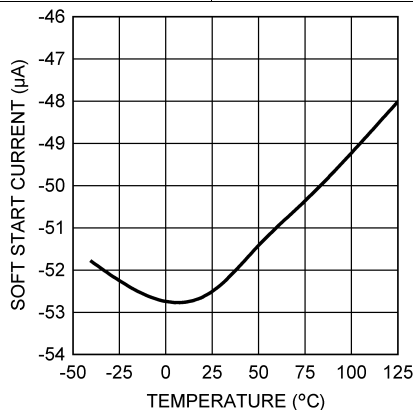
Figure 11. Soft-Start Current vs Temperature
