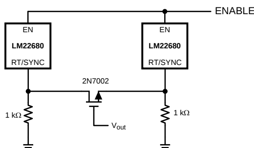
Figure 14. Self Synchronizing Setup
