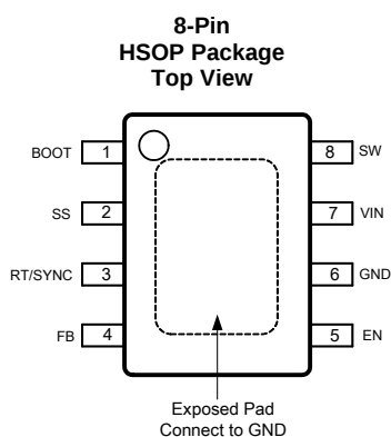
Pin Functions
