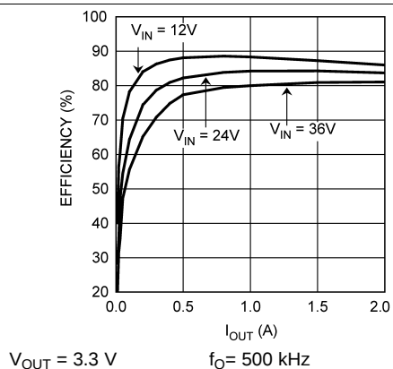
Figure 1. Efficiency vs I_{OUT} and V_{IN}
