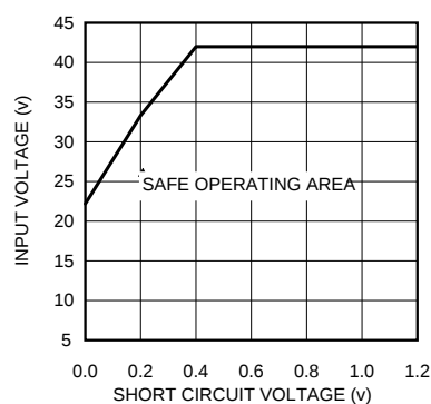
Figure 17. SOA at 500 kHz
