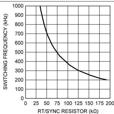
Figure 10. Switching Frequency vs RT/SYNC Resistor
