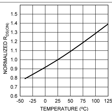
Figure 4. Normalized R_{DS(ON)} vs Temperature
