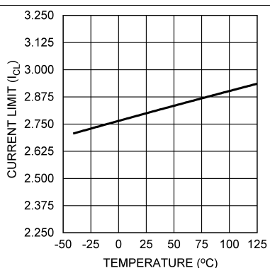
Figure 3. Current Limit vs Temperature
