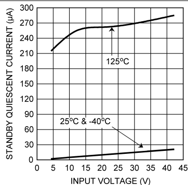
Figure 7. Standby Quiescent Current vs Input Voltage
