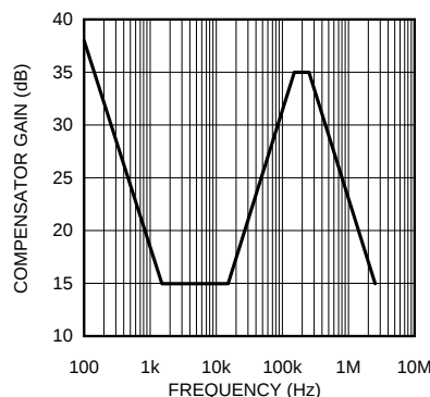
Figure 15. Compensator Gain
