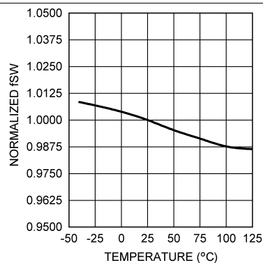
Figure 2. Normalized Switching Frequency vs Temperature
