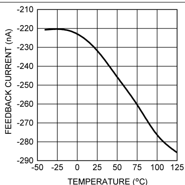
Figure 5. Feedback Bias Current vs Temperature
