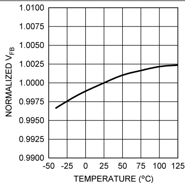
Figure 8. Normalized Feedback Voltage vs Temperature
