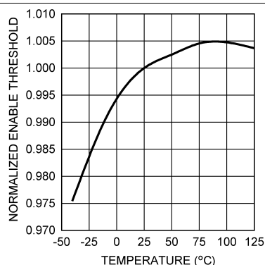
Figure 6. Normalized Enable Threshold Voltage vs Temperature
