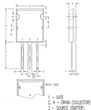
PLUS264™ (IXFB) Outline
