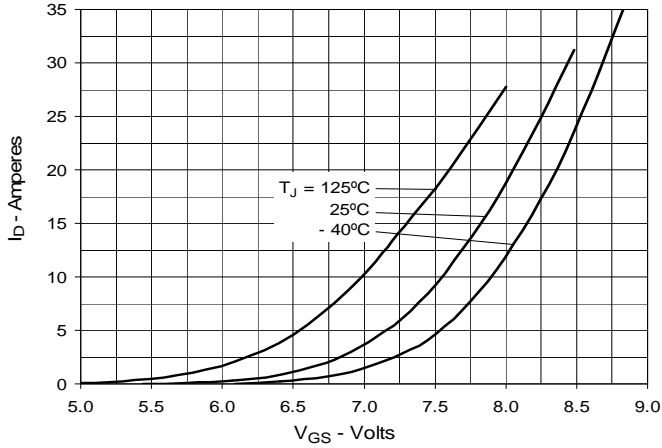
Fig. 7. Input Admittance
