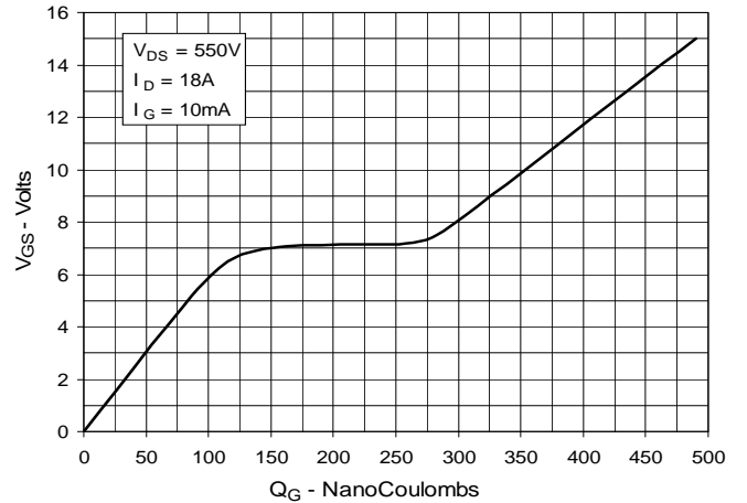
Fig. 10. Gate Charge
