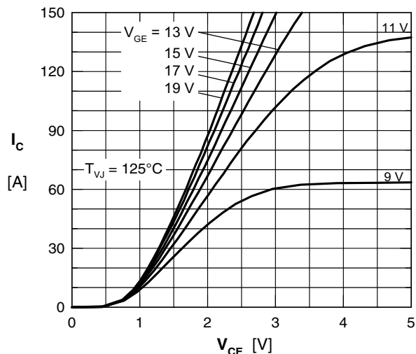
Fig. 2 output characteristics
