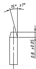
Detail Z
