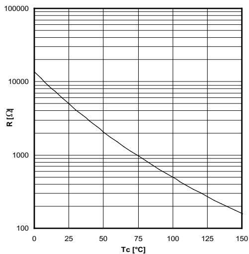
Fig. 13 Typ. NTC resistance vs. temperature
