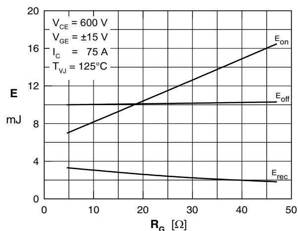
Fig. 6 Typ. switching energy vs. gate resistance
