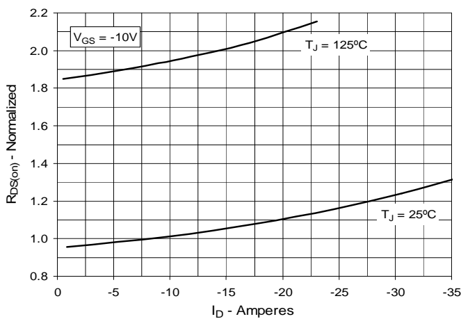
Fig. 5. R_{DS(on)} Normalized to I_D = -8\text{A} vs. Drain Current
