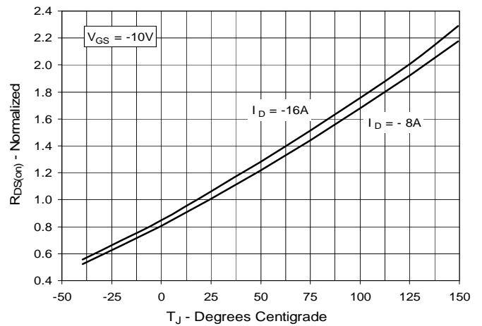
Fig. 4. R_{DS(on)} Normalized to I_D = -8\text{A} vs. Junction Temperature
