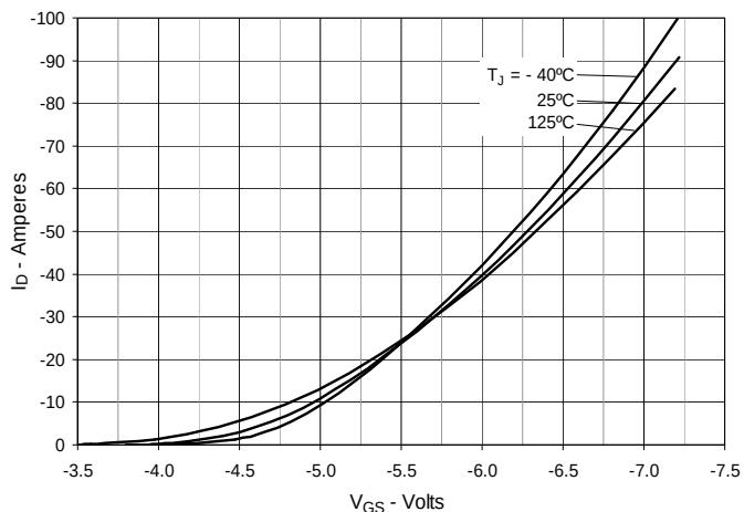
Fig. 7. Input Admittance
