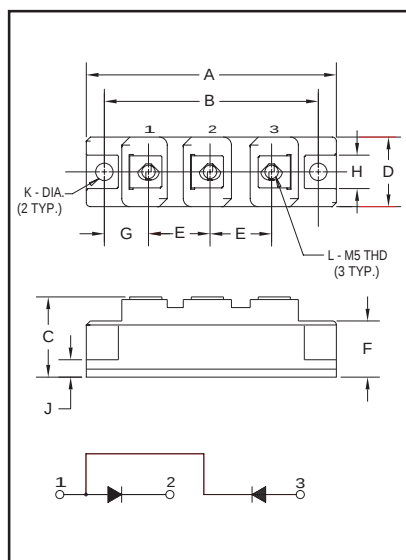
Outline Drawing
