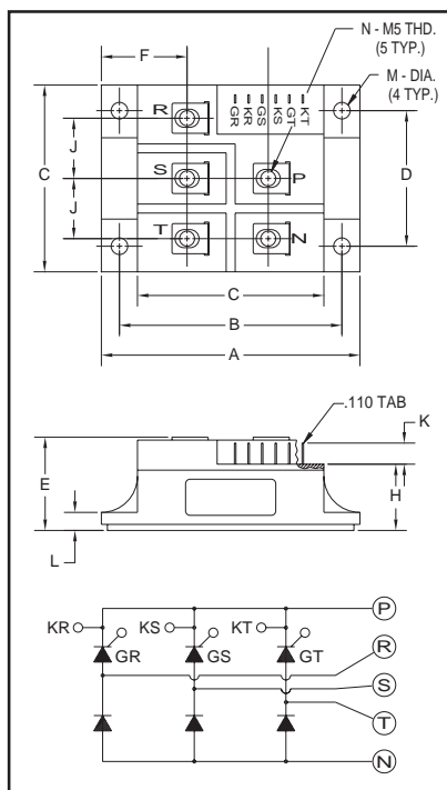
Outline Drawing
