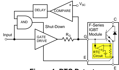
Figure 1 RTC Detector
