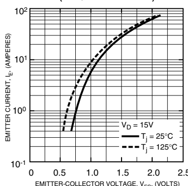
FREE-WHEEL DIODE FORWARD CHARACTERISTICS (TYPICAL - BRAKE PART)
