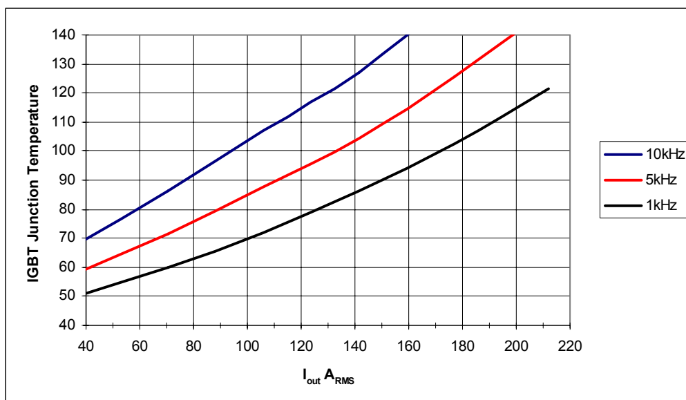
Effective Output Current vs. Carrier Frequency (Typical)
