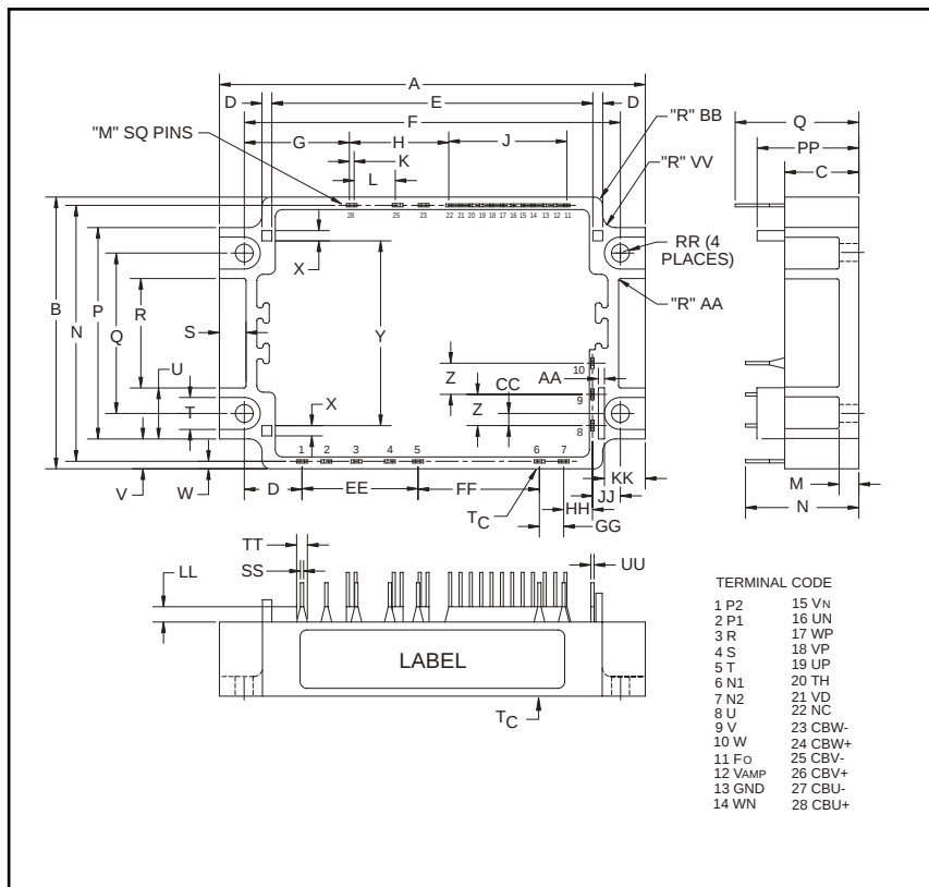
Outline Drawing and Circuit Diagram
