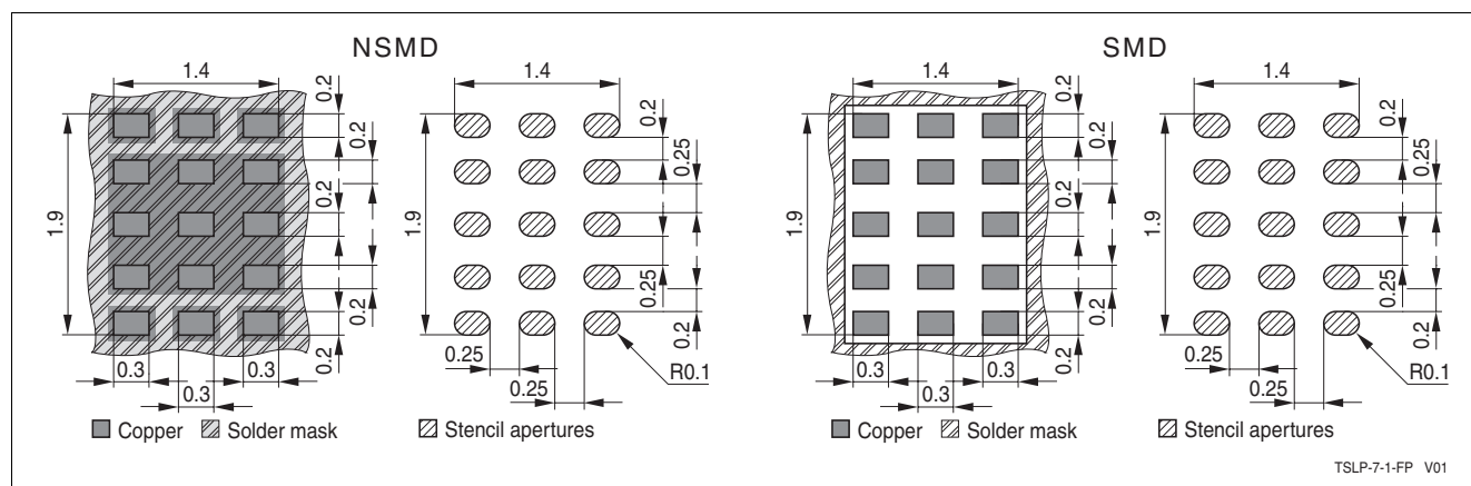
Figure 5 Footprint TSLP-7-1
