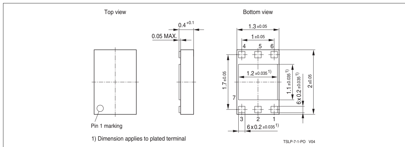
Figure 4 Package Dimensions for TSLP-7-1
