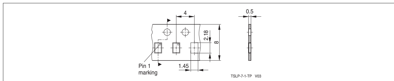
Figure 6 Tape & Reel Dimensions (Ø reel 180, pieces/reel 7500)
