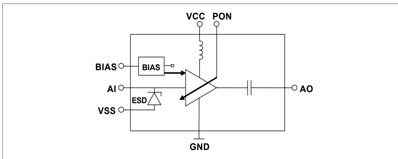
Figure 1 Blockdiagram
