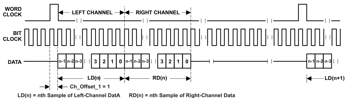
Figure 23. DSP Mode With Ch_Offset_1 = 1
