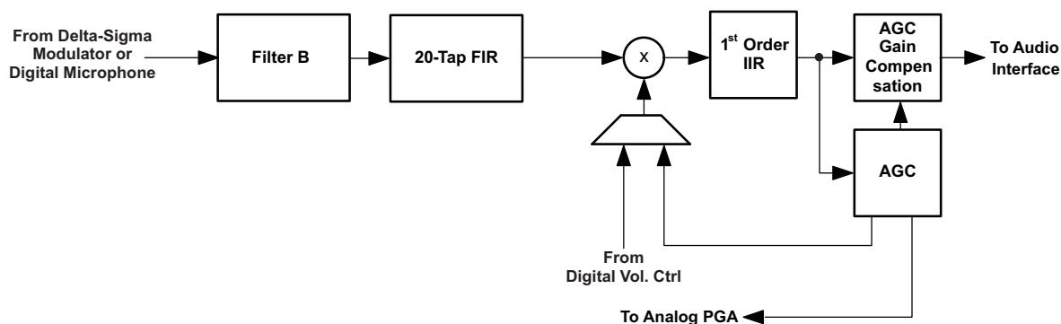
Figure 35. Signal Chain for PRB_R9 and PRB_R12
