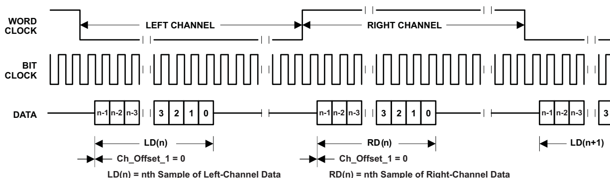
Figure 19. I²S Mode (Standard Timing)
