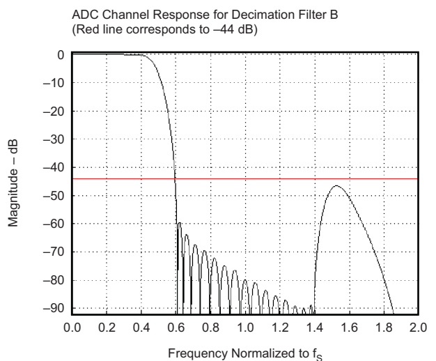
Figure 40. ADC Decimation Filter B, Frequency Response
