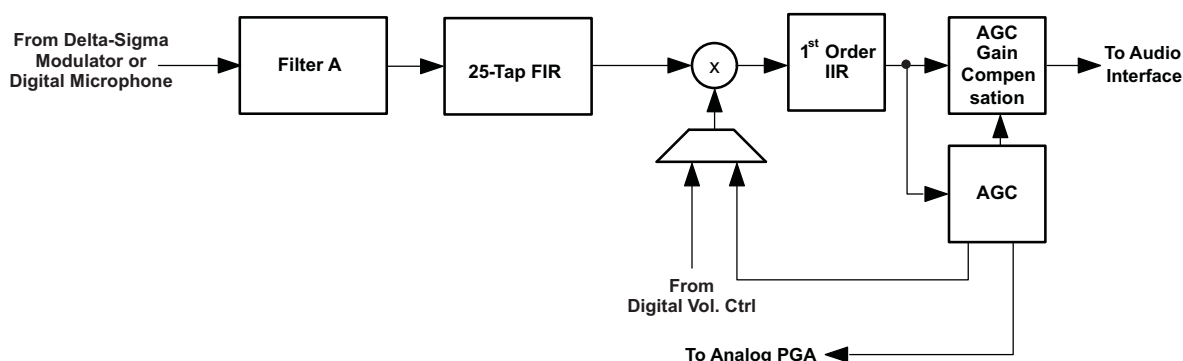
Figure 32. Signal Chain for PRB_R3 and PRB_R6
