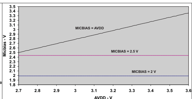
Figure 6. MICBIAS Output Voltage vs AVDD
