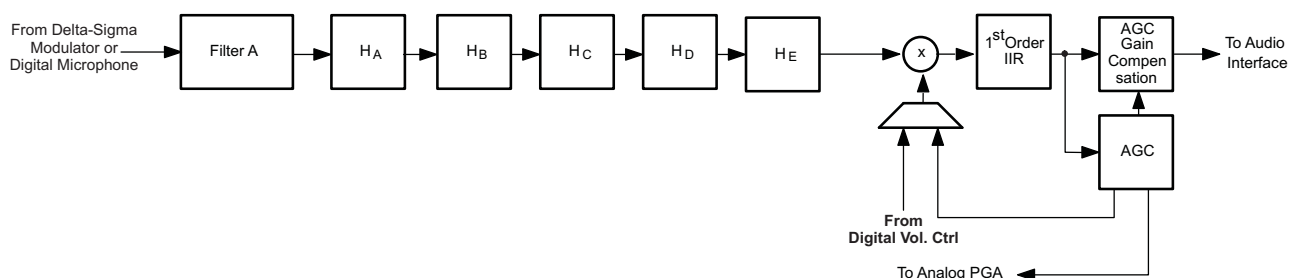
Figure 31. Signal Chain for PRB_R2 and PRB_R5
