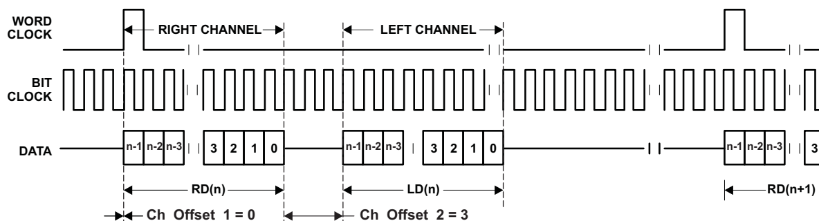
Figure 25. DSP Mode, Time-Slot-Based Mode Enabled, \text{Ch\_Offset}_1 = 0 , \text{Ch\_Offset}_2 = 3
