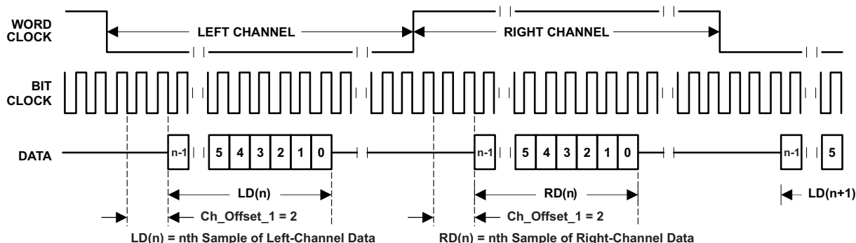
Figure 20. I²S Mode With Ch_Offset_1 = 2
