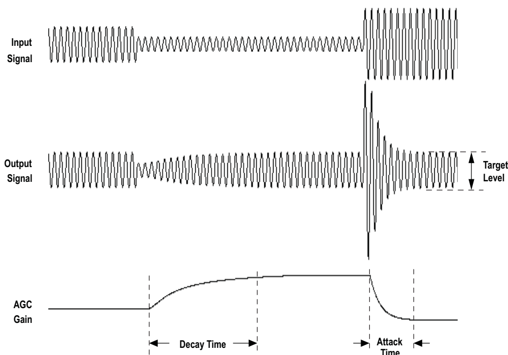
Figure 28. AGC Characteristics
