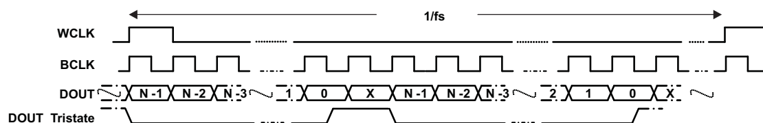
Figure 10. Both Channels Enabled, Early Hi-Z State Enabled
