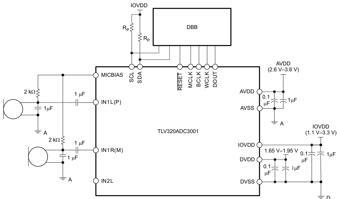
Figure 44. Typical Connections
