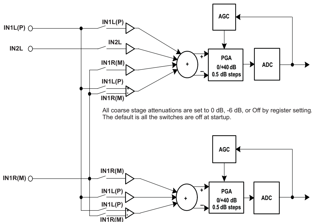
Figure 29. TLV320ADC3001 Available Audio Input Path Configurations
