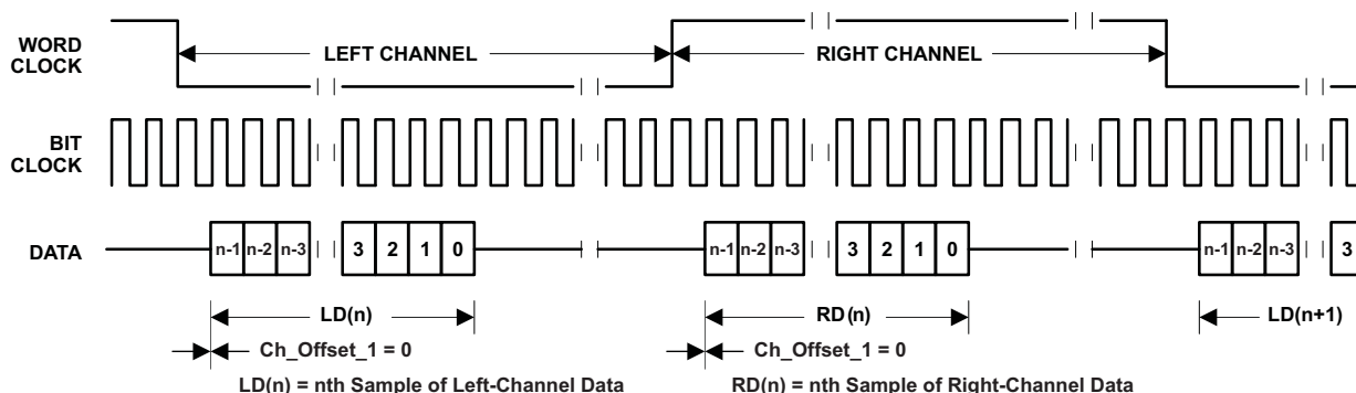
Figure 21. I²S Mode With Ch_Offset_1 = 0, Bit Clock Inverted
