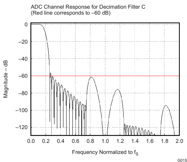
Figure 41. ADC Decimation Filter C, Frequency Response
