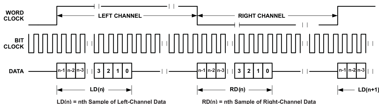
Figure 13. Left-Justified Mode (Standard Timing)
