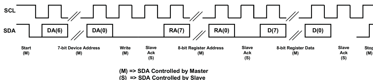
Figure 42. I 2 C Write
