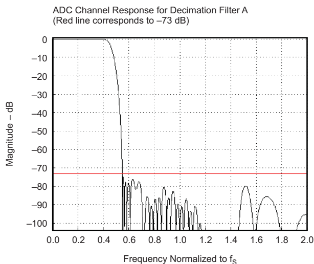
Figure 39. ADC Decimation Filter A, Frequency Response
