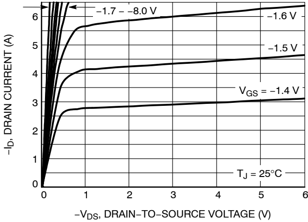
Figure 3. On-Region Characteristics
