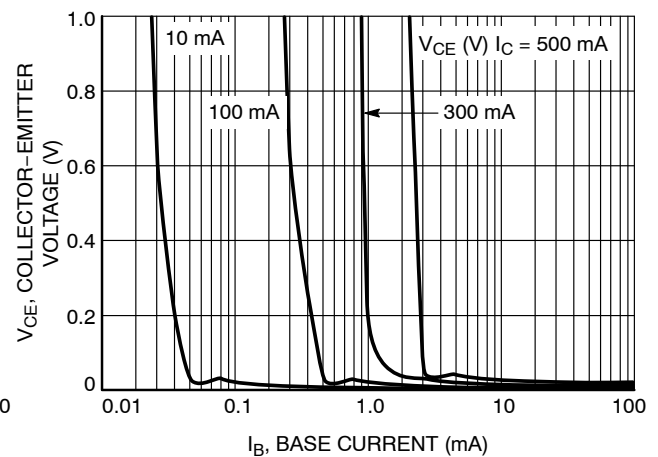
Figure 20. Saturation Region
