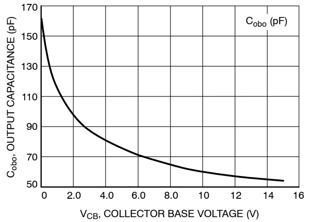
Figure 22. Output Capacitance
