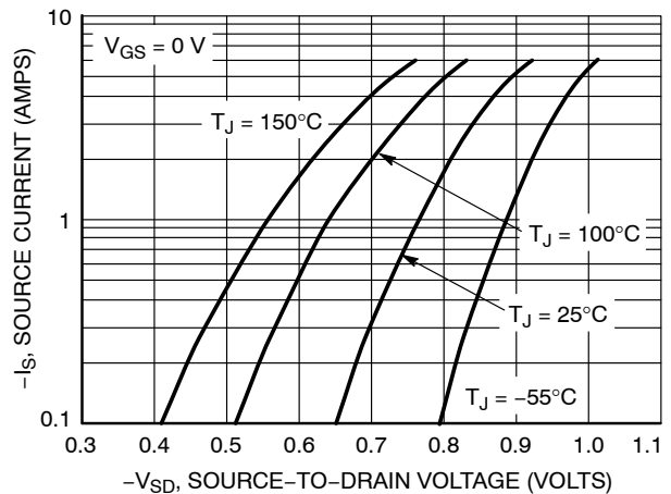
Figure 30. Diode Forward Voltage vs. Current
