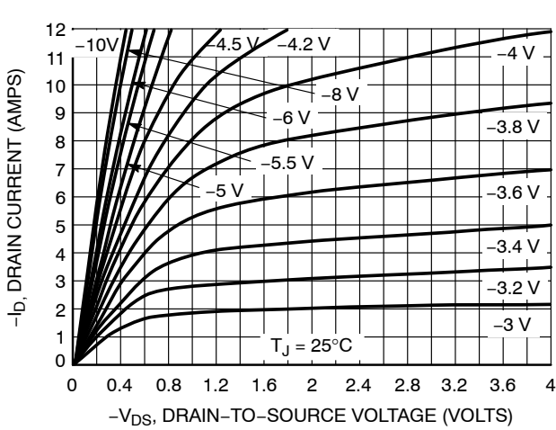
Figure 27. On-Region Characteristics
