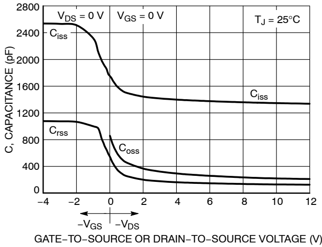
Figure 9. Capacitance Variation
