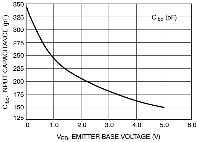
Figure 21. Input Capacitance
