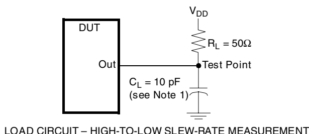
LOAD CIRCUIT – HIGH-TO-LOW SLEW-RATE MEASUREMENT
