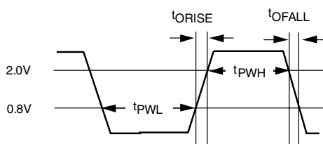
TTL Output Waveform
