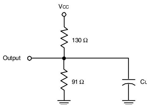
Test Load
