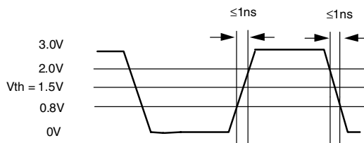
TTL Input Test Waveform
