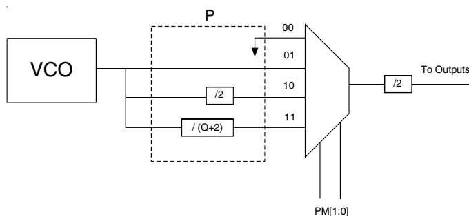
Post-Divider Diagram
