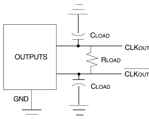
LVDS: - 100Ω between differential outputs with 5pF
