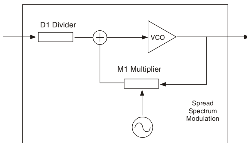
PLL1 Block Diagram
