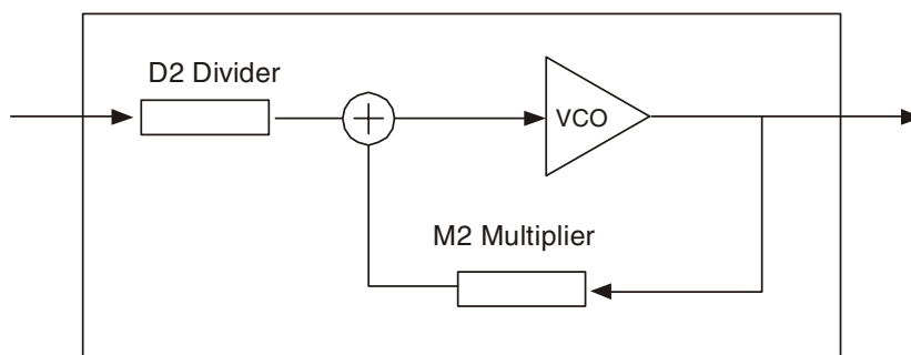
PLL2 Block Diagram
