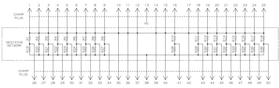
ELECTRICAL SCHEMATIC \Delta
