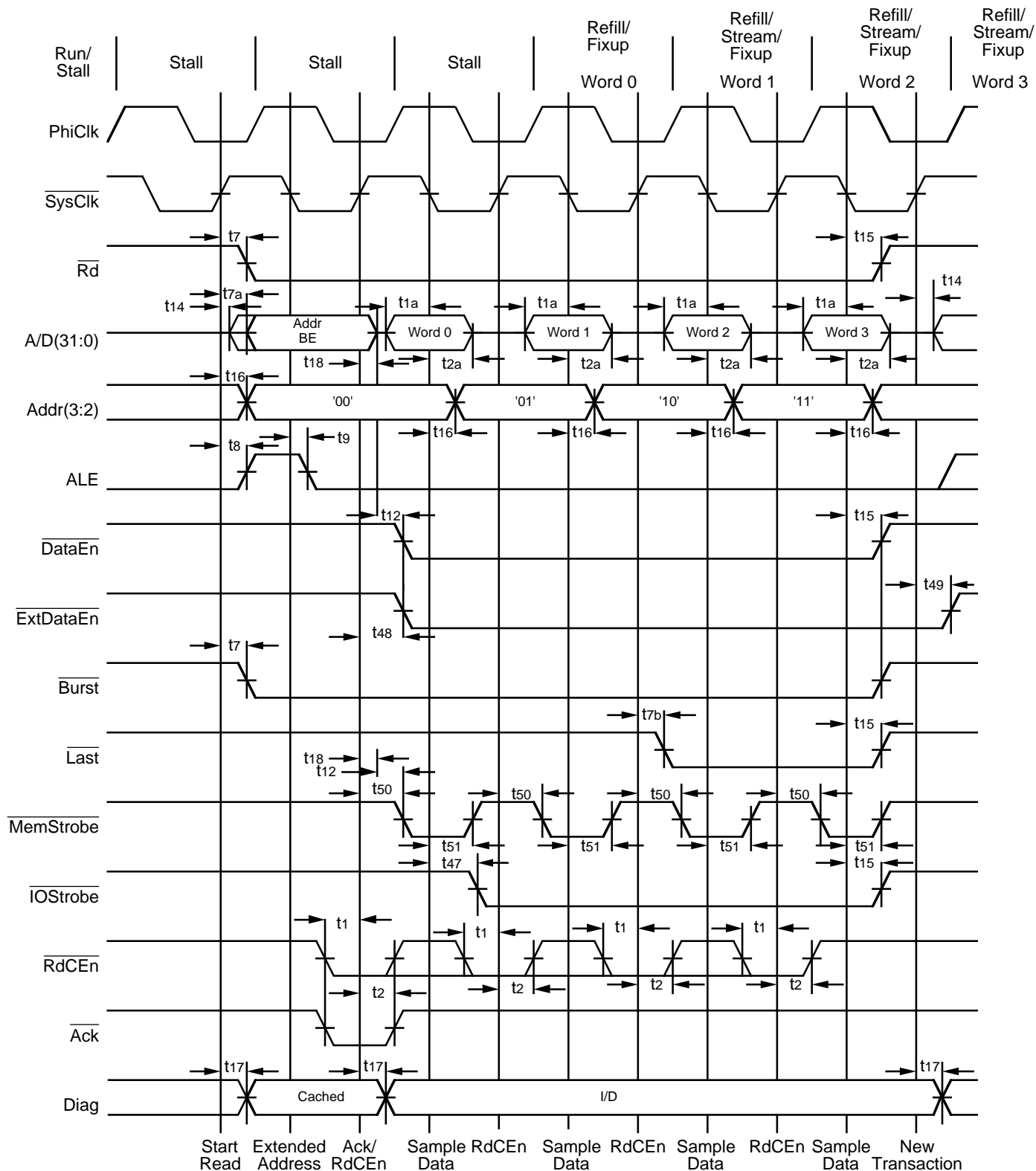
Figure 15. R3041 Quad Word Read
