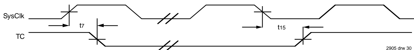
Figure 25. \overline{TC} Output
