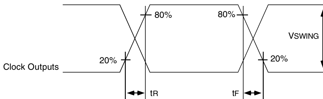
Input and Output Rise and Fall Time
