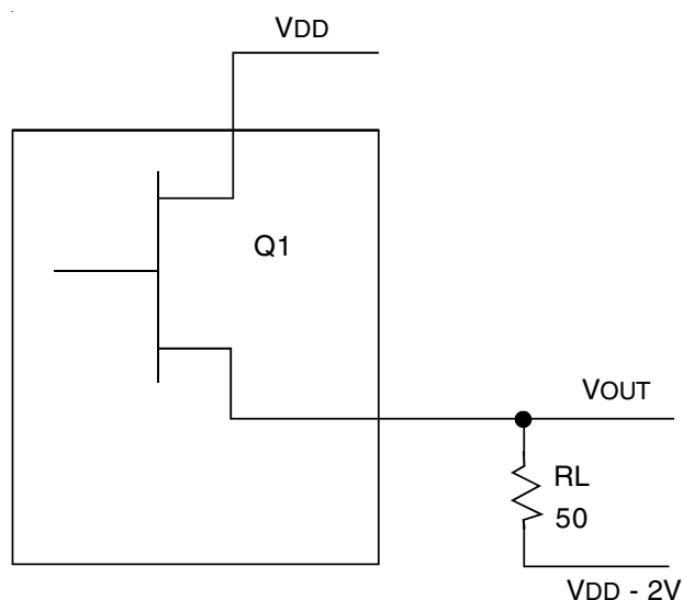
LVPECL Output Driver Circuit and Termination
