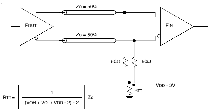
LVPECL Output Termination, layout A
