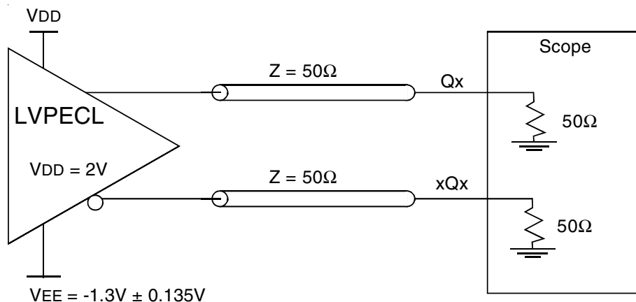
Output Load Test Circuit
