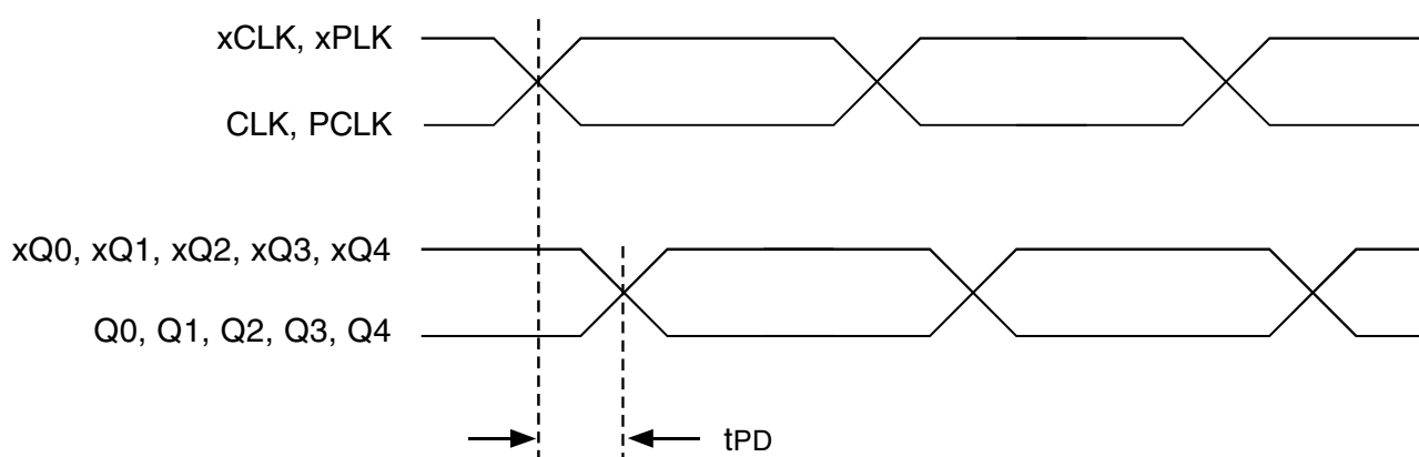
Propagation Delay
