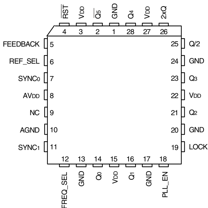
PLCC TOP VIEW
