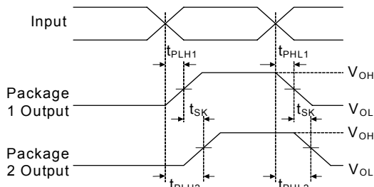
Figure 5. Part-to-Part Skew
