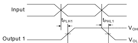
Figure 4. Pulse Skew ( t_{SK(p)} = |t_{PLH} - t_{PH}| )
