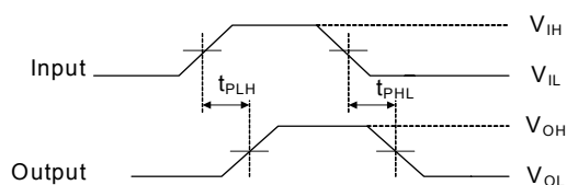
Figure 2. Propagation Delay
