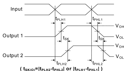
Figure 3. Output Skew
