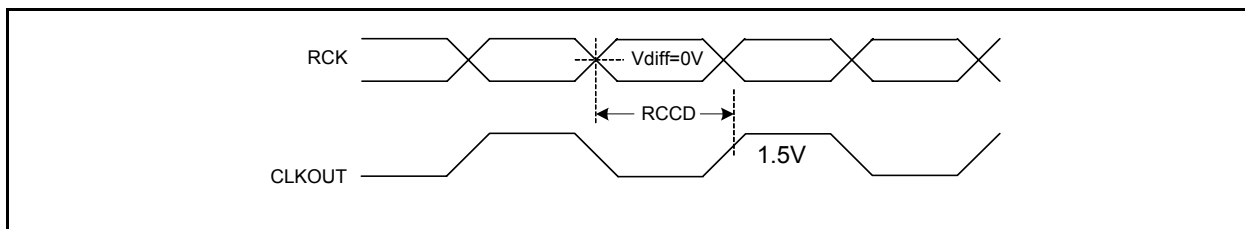
Figure 4. V386 Clock In to Clock Out Delay
