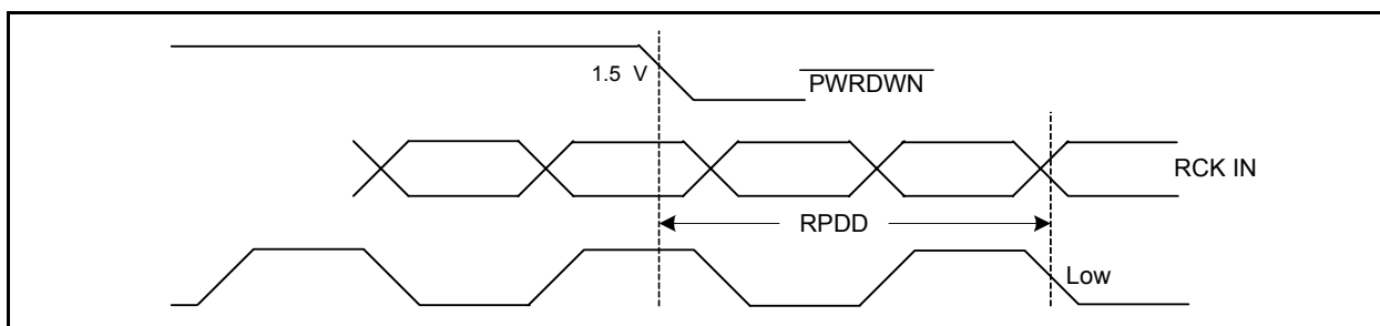
Figure 6. V386 Power Down Delay
