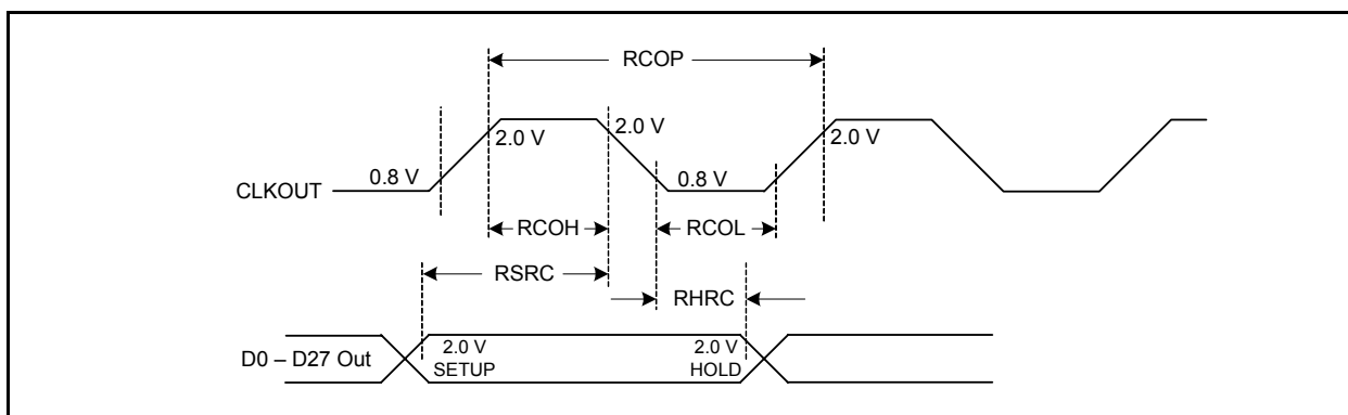
Figure 3. V386 SETUP/HOLD and High/Low Times
