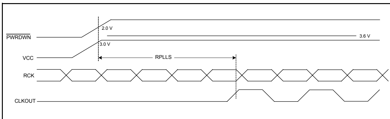
Figure 5. V386 Phase Lock Loop Set Time
