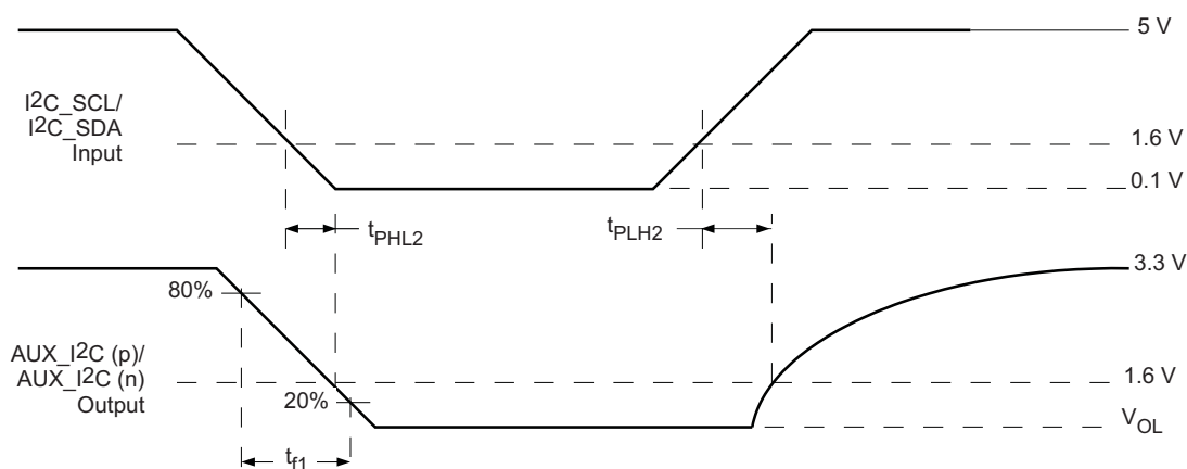
Figure 16. Source Side Output AC Measurements
