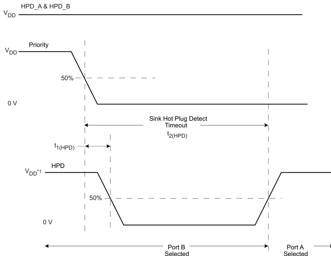
Figure 3. HPD Timing Diagram #2
