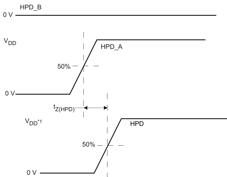
Figure 4. HPD Timing Diagram #3
