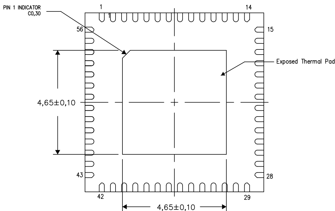
Bottom View
