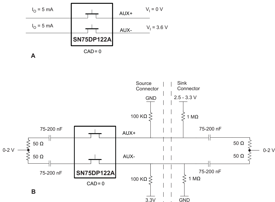
Figure 5. Auxiliary Channel Test Circuit (CAD = LOW)
