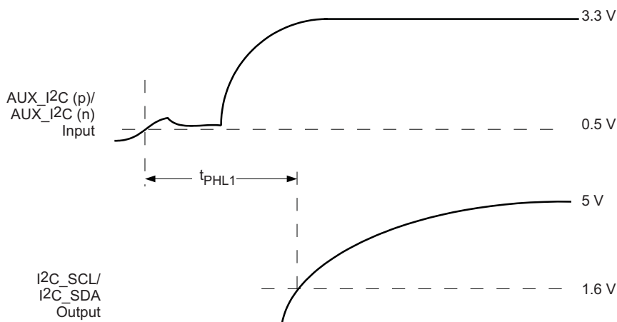
Figure 18. Sink Side Output AC Measurements Continued
