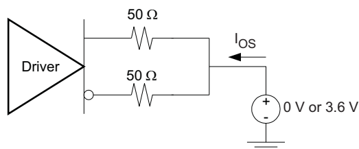
Figure 23. TMDs Main Link Short Circuit Output Circuit
