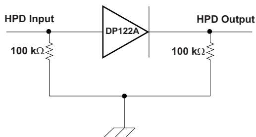
Figure 1. HPD Test Circuit
