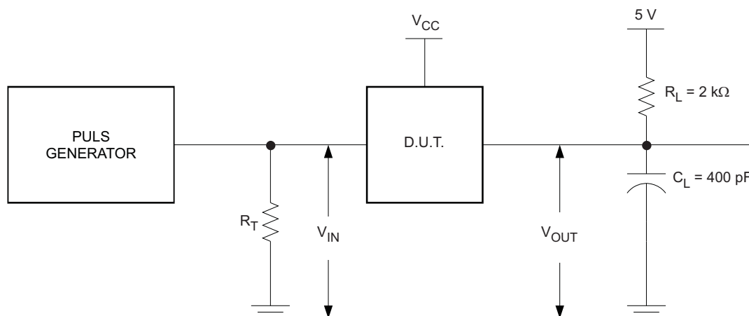
Figure 15. Sink Side Test Circuit (SCL, SDA)
