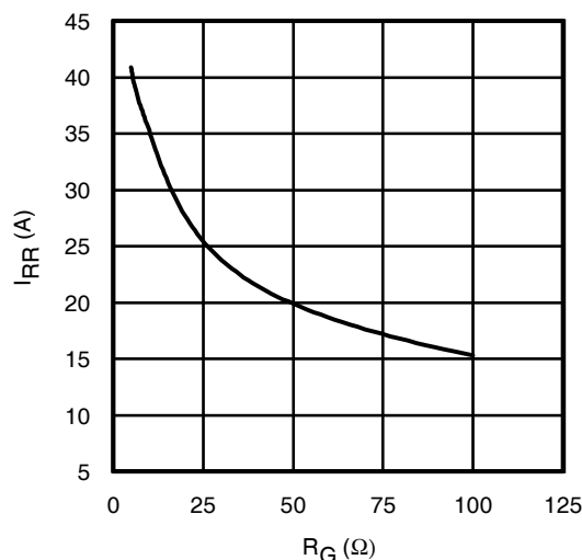
Fig. 18 - Typ. Diode I_{RR} vs. R_G T_J = 175^\circ\text{C}
