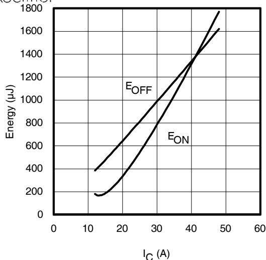
Fig. 13 - Typ. Energy Loss vs. I_C
