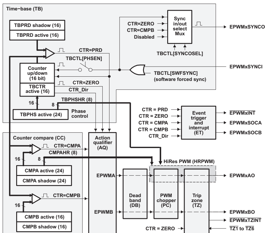
Figure 4-5. ePWM Submodules Showing Critical Internal Signal Interconnections
