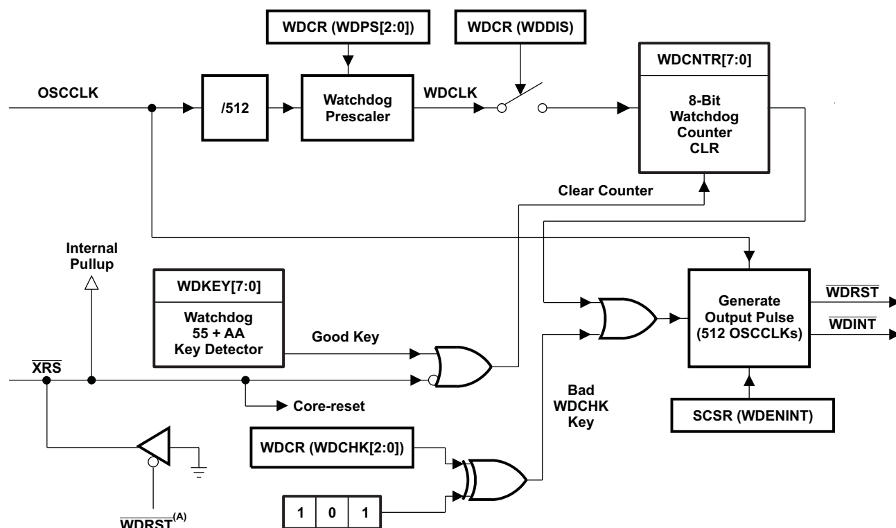
Figure 3-13. Watchdog Module
