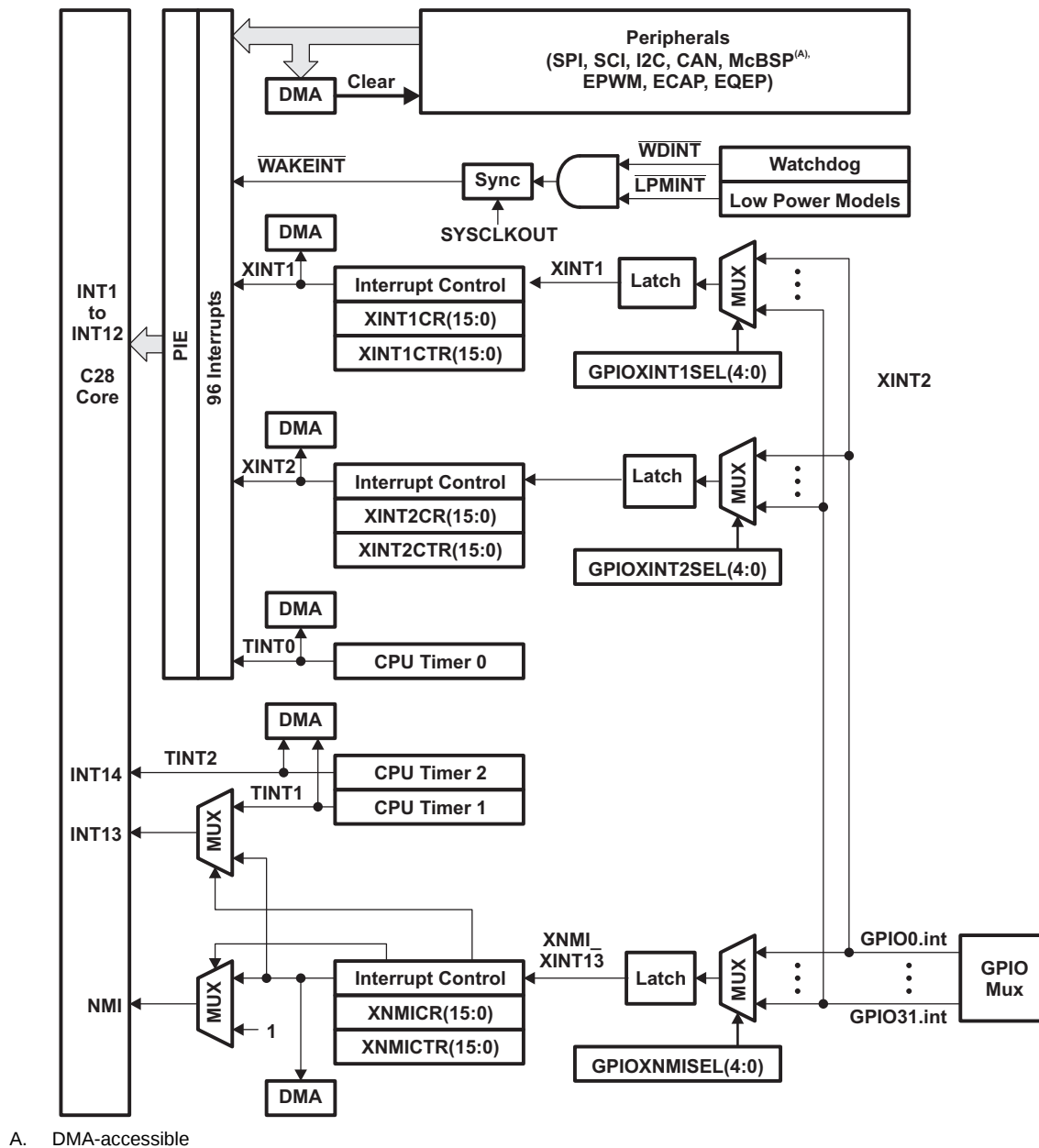
Figure 3-5. External and PIE Interrupt Sources
