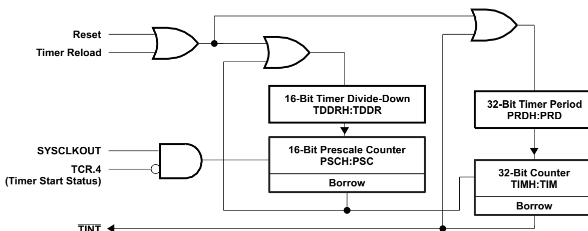
Figure 4-2. CPU-Timers
