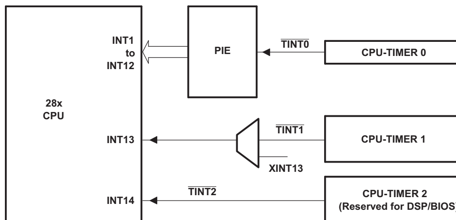
Figure 4-3. CPU-Timer Interrupt Signals and Output Signal
