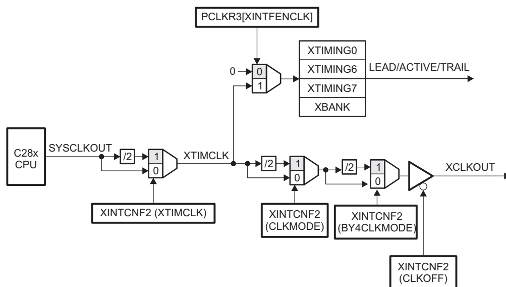
Figure 6-21. Relationship Between XTIMCLK and SYSCLKOUT
