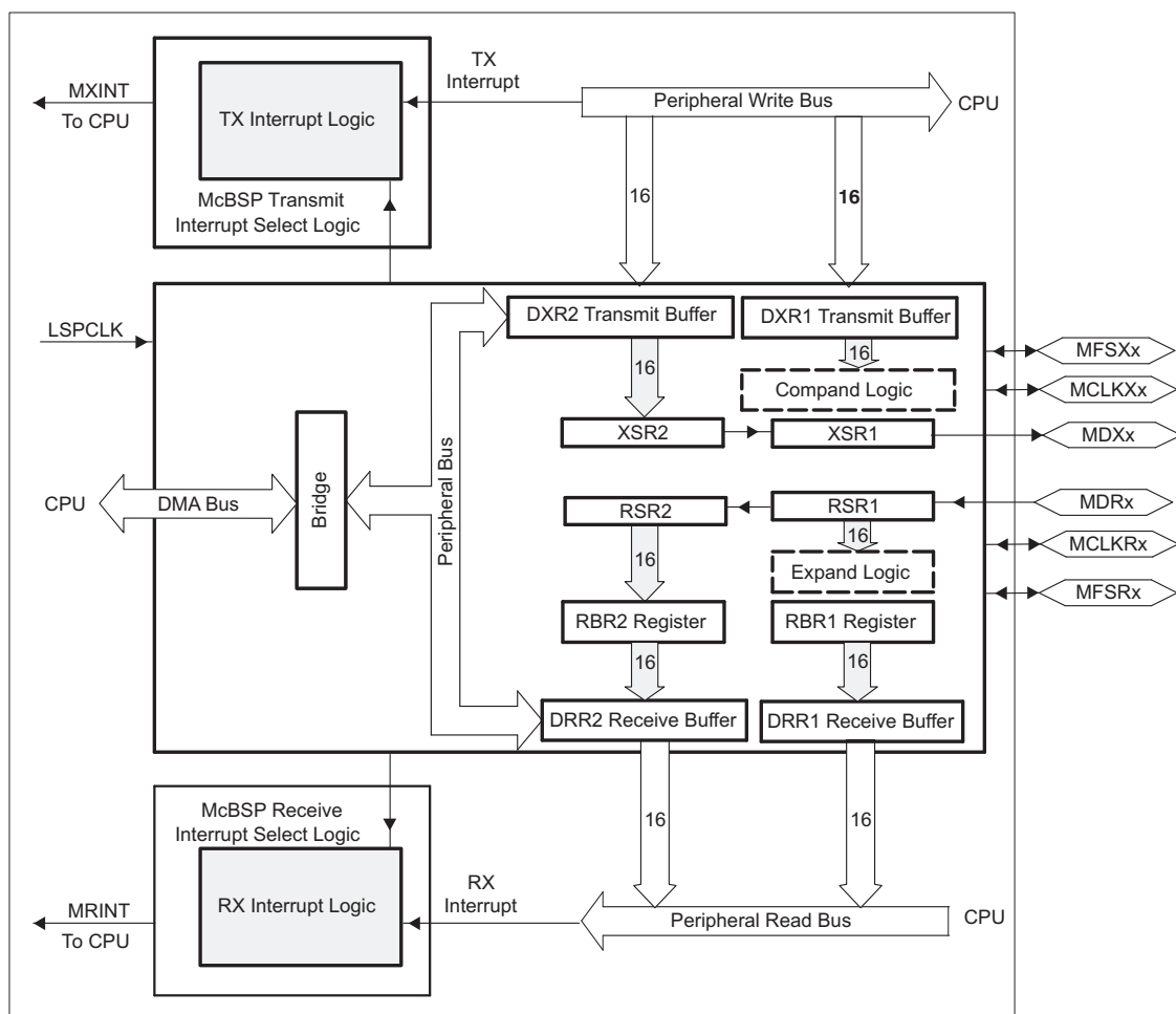
Figure 4-9. McBSP Module
