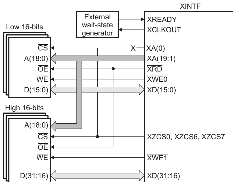
Figure 4-20. Typical 32-bit Data Bus XINTF Connections
