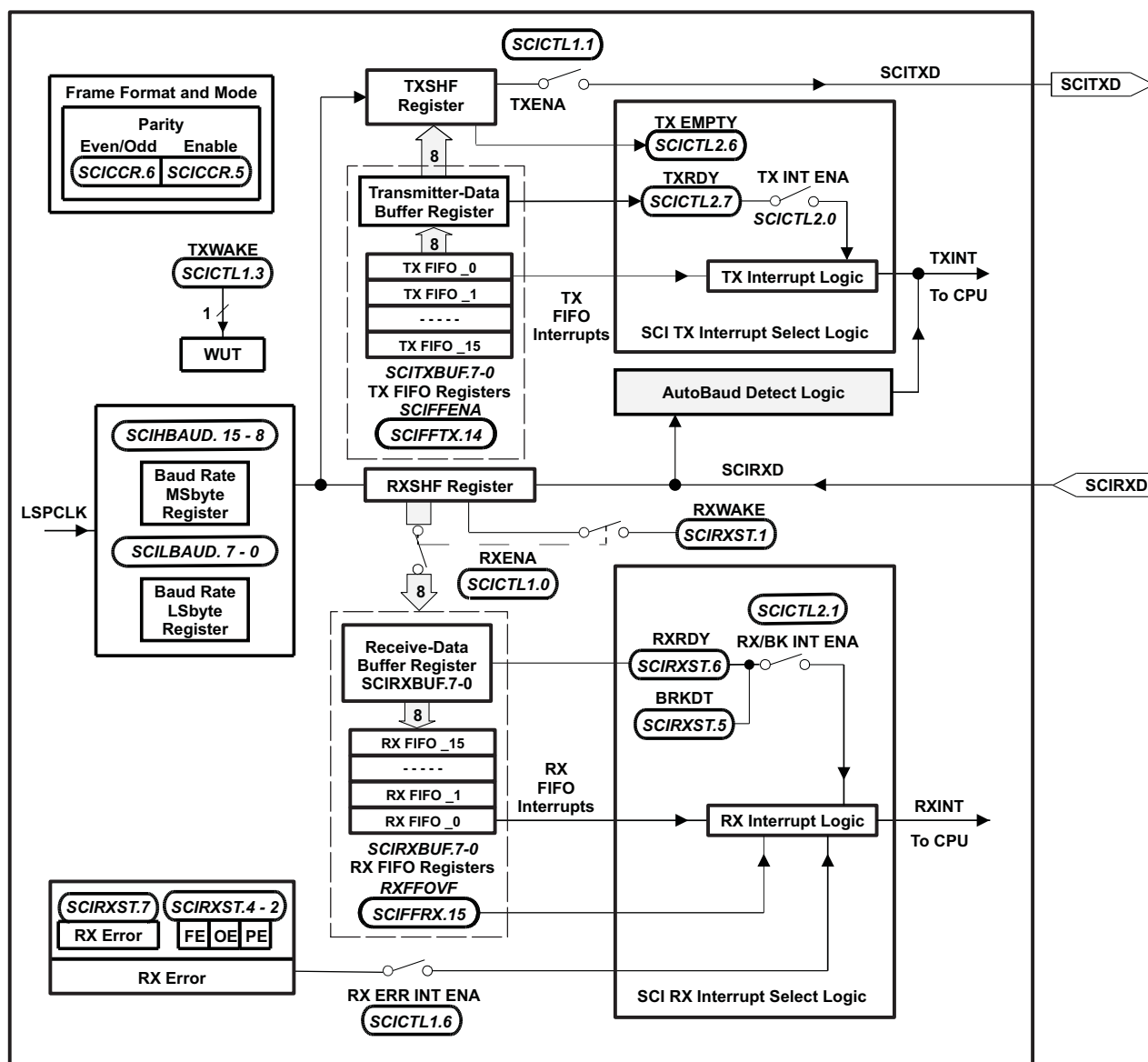
Figure 4-13. Serial Communications Interface (SCI) Module Block Diagram
