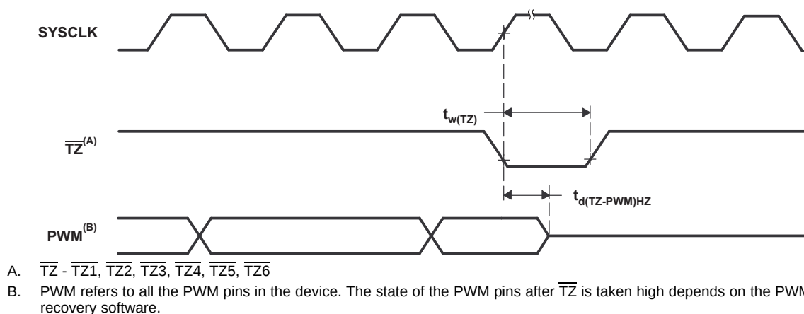
Figure 6-14. PWM Hi-Z Characteristics
