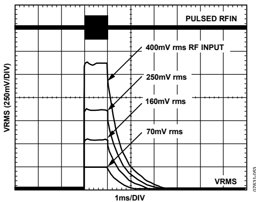
Figure 53. Output Response to Various RF Input Pulse Levels, Supply 3 V, 900 MHz Frequency, Square-Domain Filter Open, Output Filter 0.1 µF
