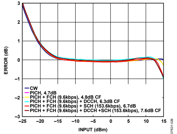
Figure 26. Error from CW Linear Reference vs. Input with Various CDMA2000 Reverse Link Waveforms at 1900 MHz, C_{FLTR} = 10\text{ nF} , C_{OUT} = \text{Open}
