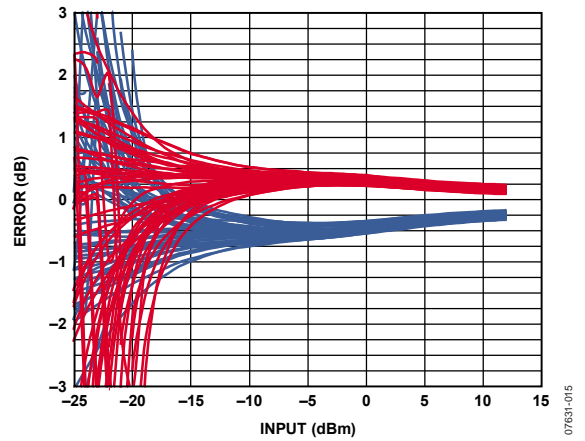
Figure 15. VRMS Output Delta from +25°C Output Voltage for 50 Devices at -40°C and +85°C, 3500 MHz Frequency
