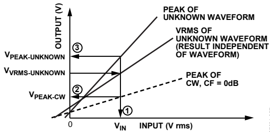
Figure 57. Procedure for Crest Factor Calculation
