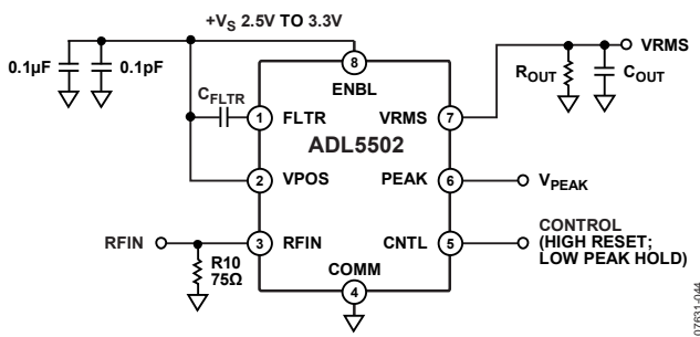
Figure 44. Basic Connections for ADL5502
