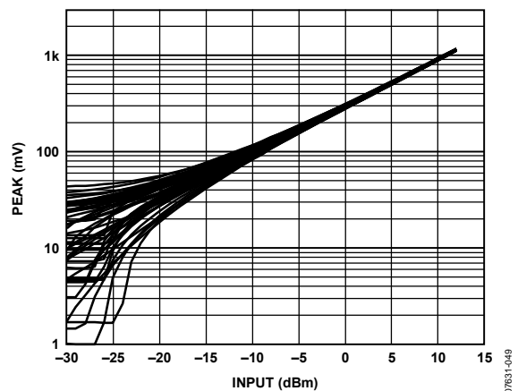
Figure 49. PEAK Output vs. Input Level Distribution of 50 Devices, 900 MHz Frequency, Supply 3.0 V
