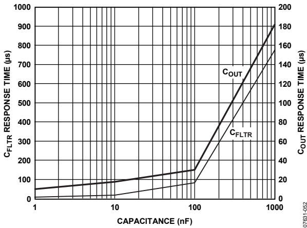
Figure 52. Response Time vs. C_{FLTR} and C_{OUT}
