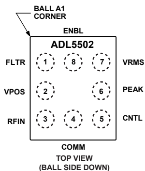
Figure 3. Pin Configuration
