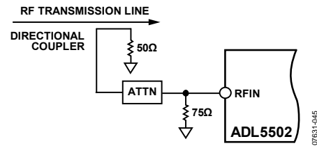
Figure 45. Input Interfacing to Directional Coupler
