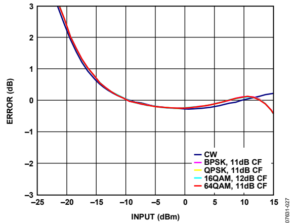
Figure 27. Error from CW Linear Reference vs. Input with Various 802.16 OFDM Waveforms at 3500 MHz, 10 MHz Signal BW, and 256 Subcarriers for All Modulated Signals, C_{FLTR} = 10\text{ nF} , C_{OUT} = \text{Open}
