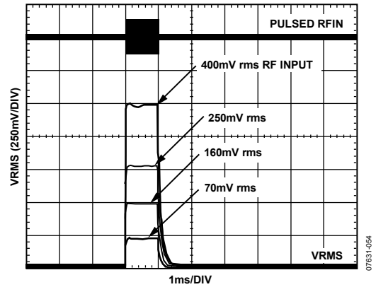
Figure 54. Output Response to Various RF Input Pulse Levels, Supply 3 V, 900 MHz Frequency, Square-Domain Filter Open, Output Filter 0.1 µF with Parallel 1 kΩ
