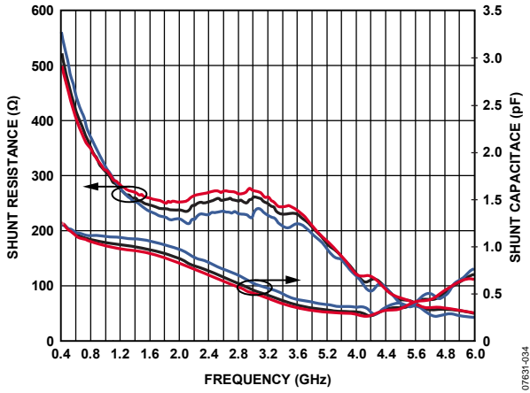
Figure 34. Input Impedance vs. Frequency, Supply 3 V, Temperatures -40°C, +25°C, and +85°C
