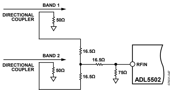
Figure 47. Combining Multiple RF Input Signals
