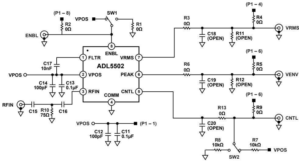
Figure 65. Evaluation Board Schematic
