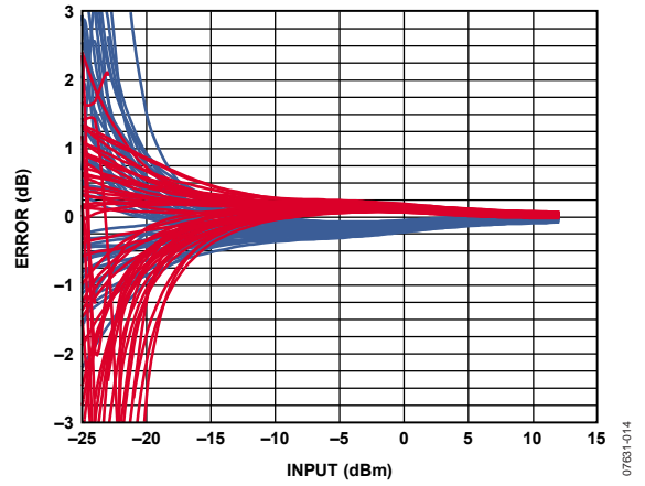
Figure 14. VRMS Output Delta from +25°C Output Voltage for 50 Devices at -40°C and +85°C, 1900 MHz Frequency
