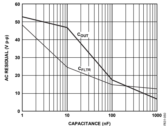
Figure 50. AC Residual vs. C_{FLTR} and C_{OUT} , W-CDMA Forward Link (4.6 dB CF) Waveform
