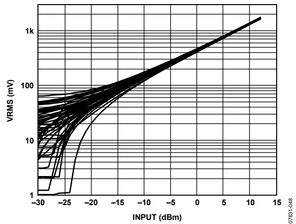
Figure 48. VRMS Output vs. Input Level Distribution of 50 Devices, 900 MHz Frequency, Supply 3.0 V
