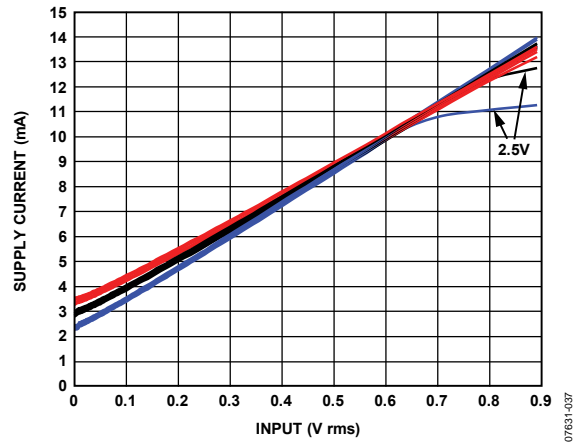
Figure 37. Supply Current vs. Input Level; 2.5 V, 3.0 V, and 3.3 V Supply; 900 MHz Frequency, Temperatures -40°C, +25°C, and +85°C
