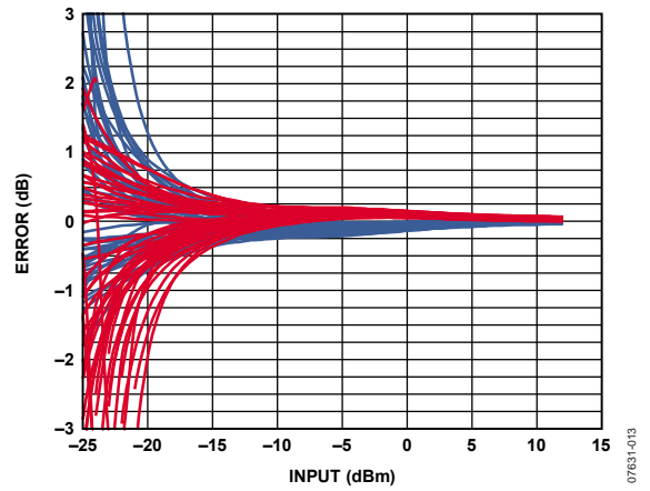
Figure 13. VRMS Output Delta from +25°C Output Voltage for 50 Devices at -40°C and +85°C, 900 MHz Frequency
