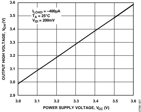
Figure 5. Output High Voltage vs. Power Supply Voltage
