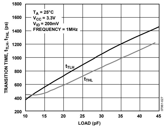
Figure 20. Transition Time vs. Load
