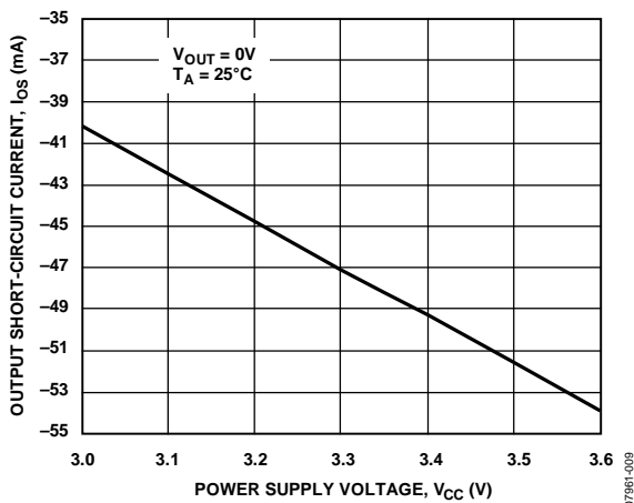
Figure 7. Output Short-Circuit Current vs. Power Supply Voltage
