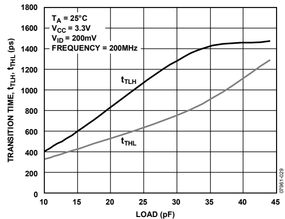
Figure 22. Transition Time vs. Load at 200 MHz
