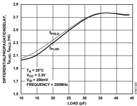
Figure 21. Differential Propagation Delay vs. Load at 200 MHz
