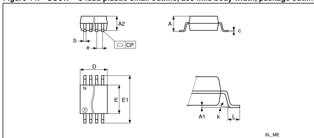
Figure 14. SO8W – 8-lead plastic small outline, 208 mils body width, package outline
