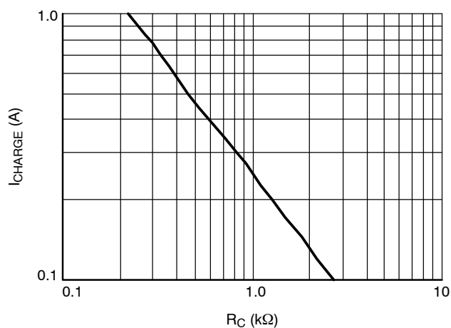
Figure 4. Charge Current vs. R C
