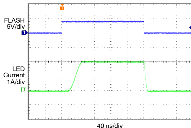
Figure 16. FLASH Transient Response
