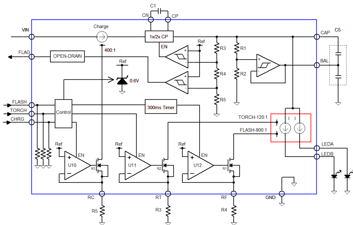
Figure 18. Functional Block Diagram
