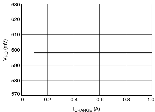
Figure 9. V RC vs. I CHARGE
