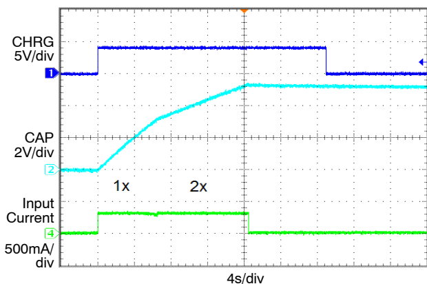
Figure 15. Charge Cycle, 300 mA Input Current
