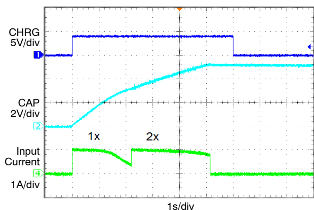
Figure 13. Charge Cycle, 1 A Input Current
