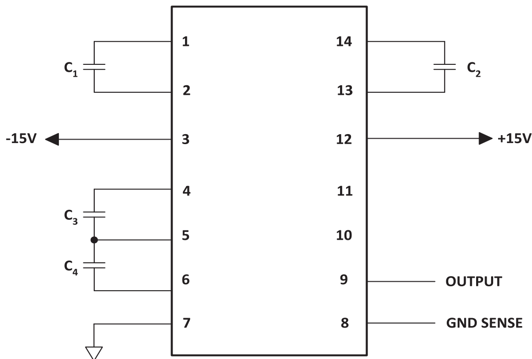
Figure 1: Typical Connection
