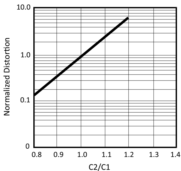
Figure 8: Normalized Distortion vs. C2/C1
