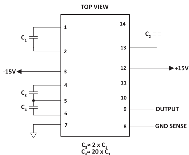
Figure 14: Extended Frequency External Connections
