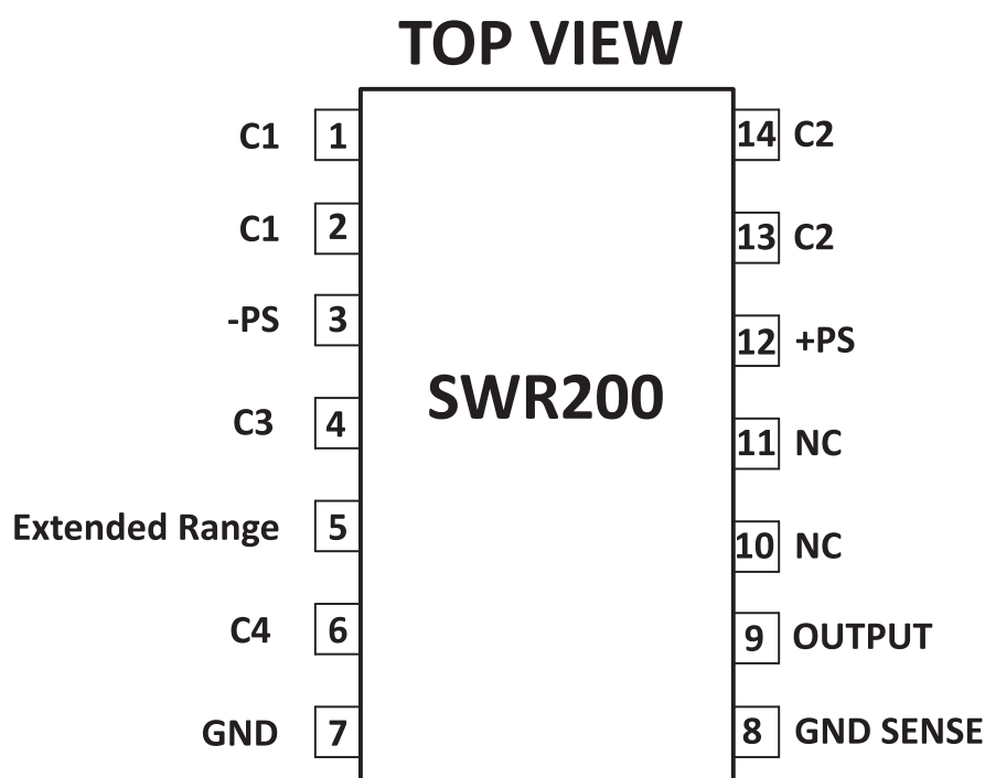
Figure 13: Pin Configuration
