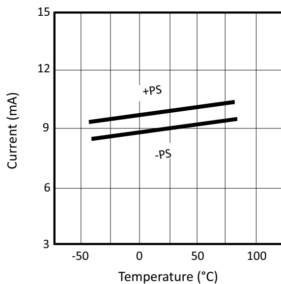
Figure 9: Power Supply Current vs. Temperature
