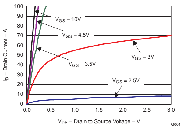
Figure 2. Saturation Characteristics
