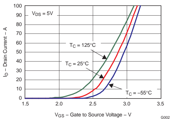
Figure 3. Transfer Characteristics
